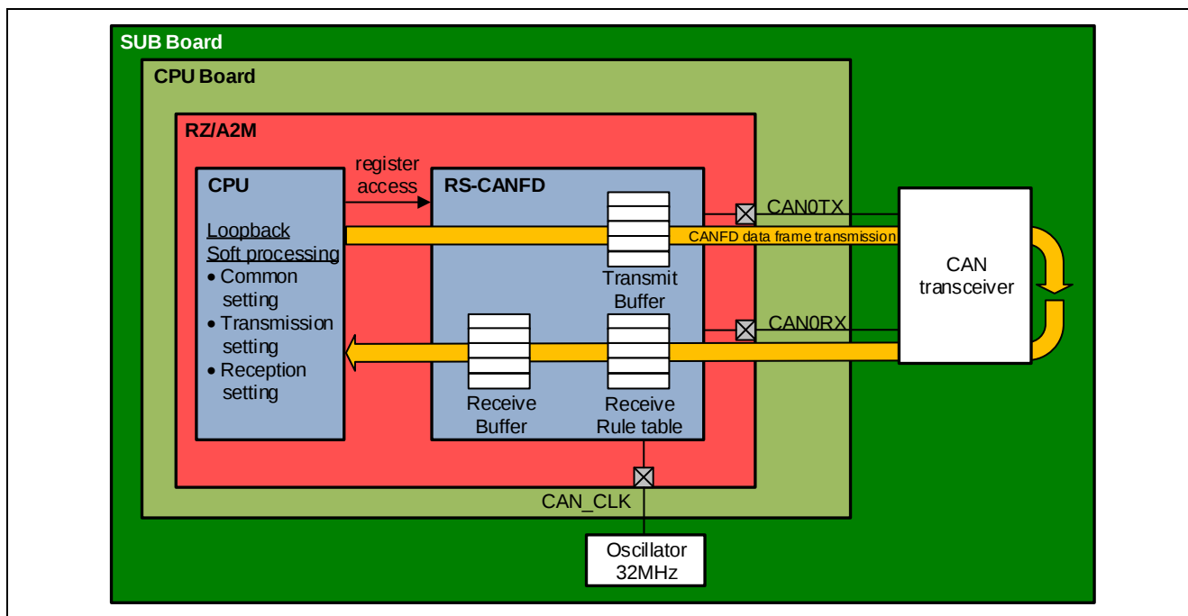
Figure 3-9 System configuration
