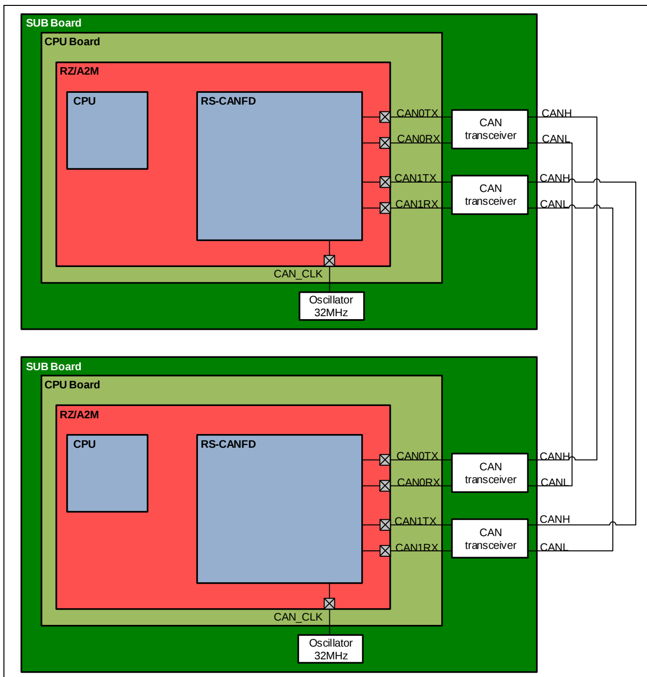
Figure 2-1 Hardware configuration
