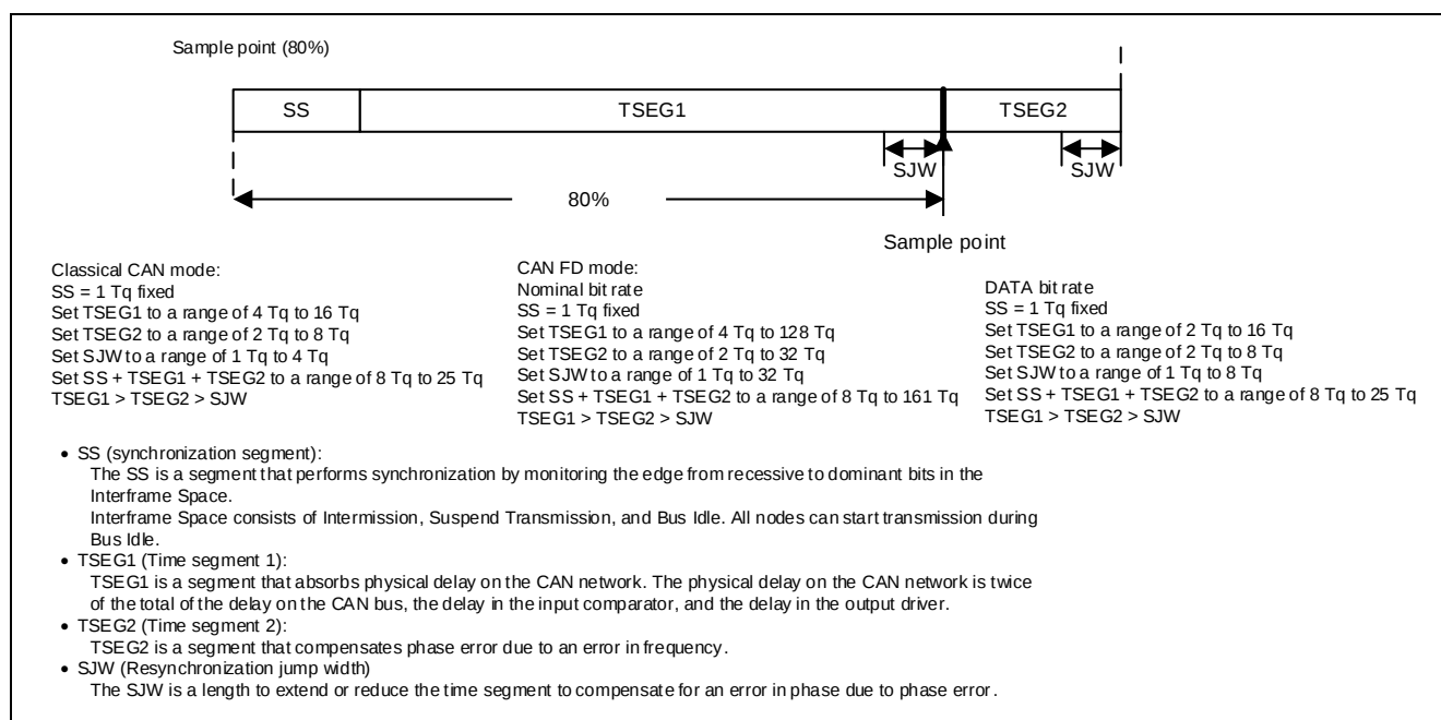
Figure 3-3 Bit segments and sample point
