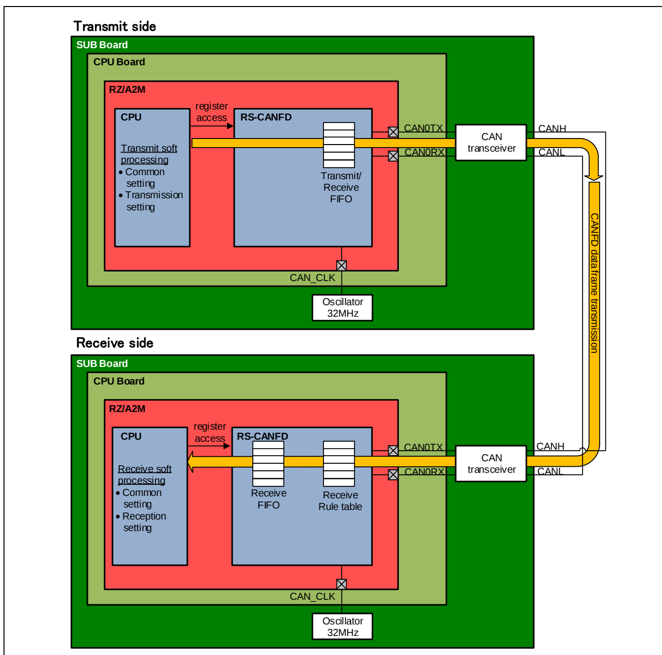
Figure 3-4 System configuration
