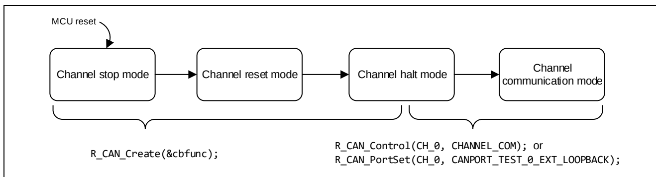
Figure 3-2 State transition diagram of the channel mode
