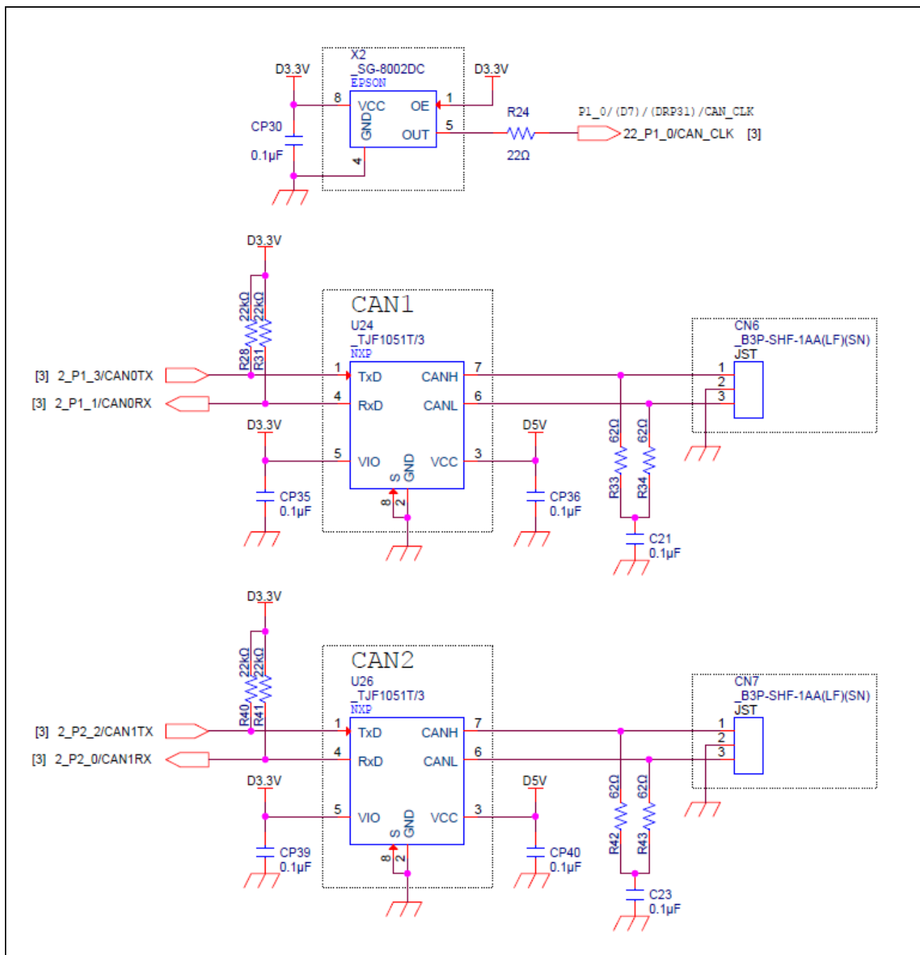
Figure 2-2 Part of the circuit diagram of the RZ/A2M SUB board
