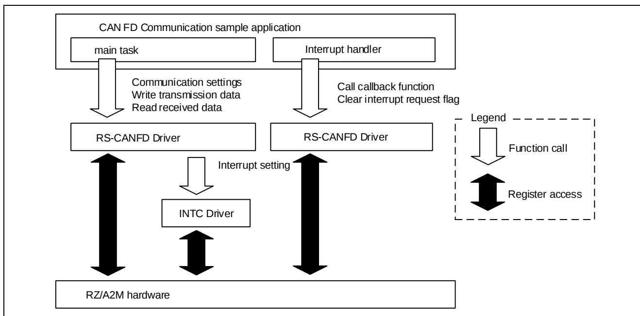
Figure 2-3 Sample program system block diagram
