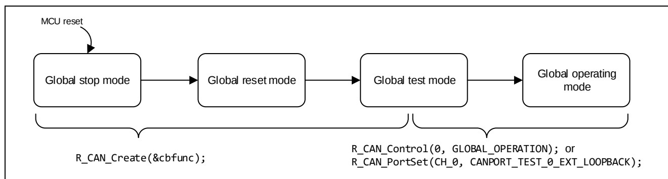
Figure 3-1 State transition diagram of the global mode
