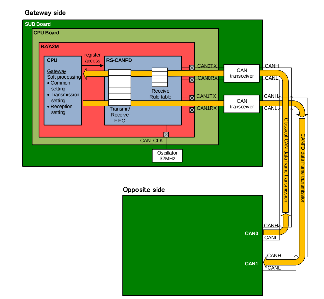
Figure 3-7 System configuration
