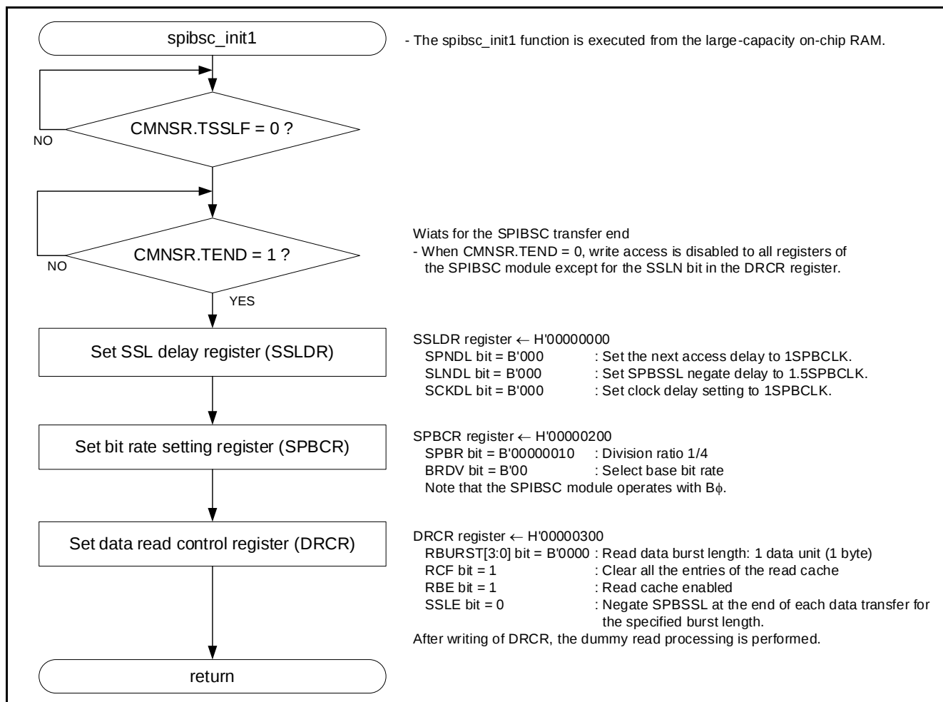
Figure 5.5 Flowchart of Loader program 1
