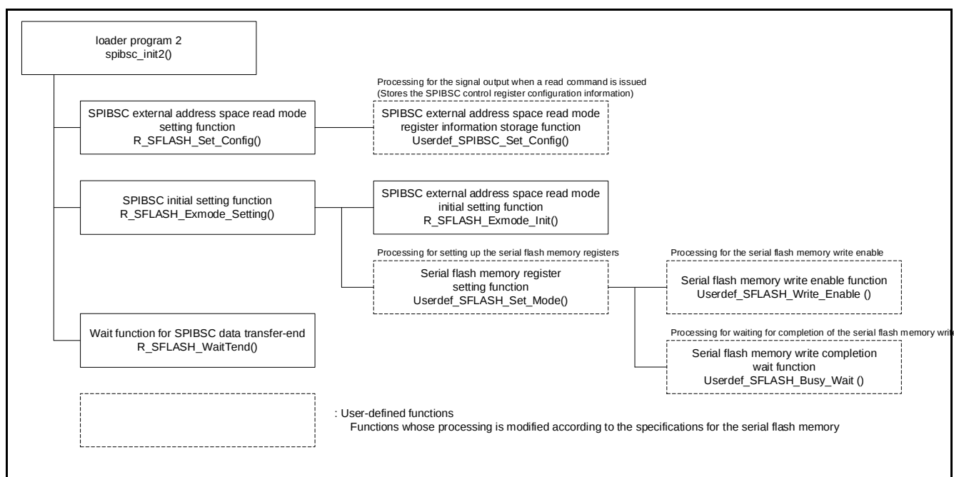
Figure 6.4 Hierarchical Module Diagram of the Loader program 2
