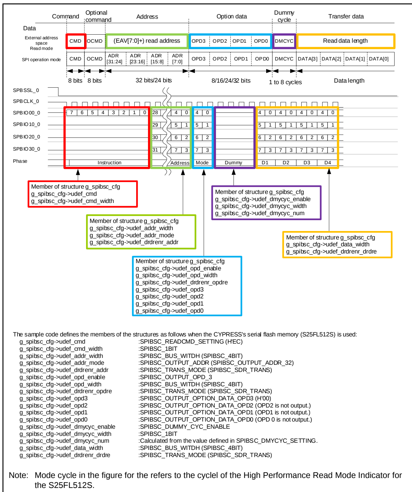
Figure 6.5 Correspondence between SPIBSC Control Register Settings and Waveforms Output to Serial Flash Memory during SPIBSC External Address Read Operation
