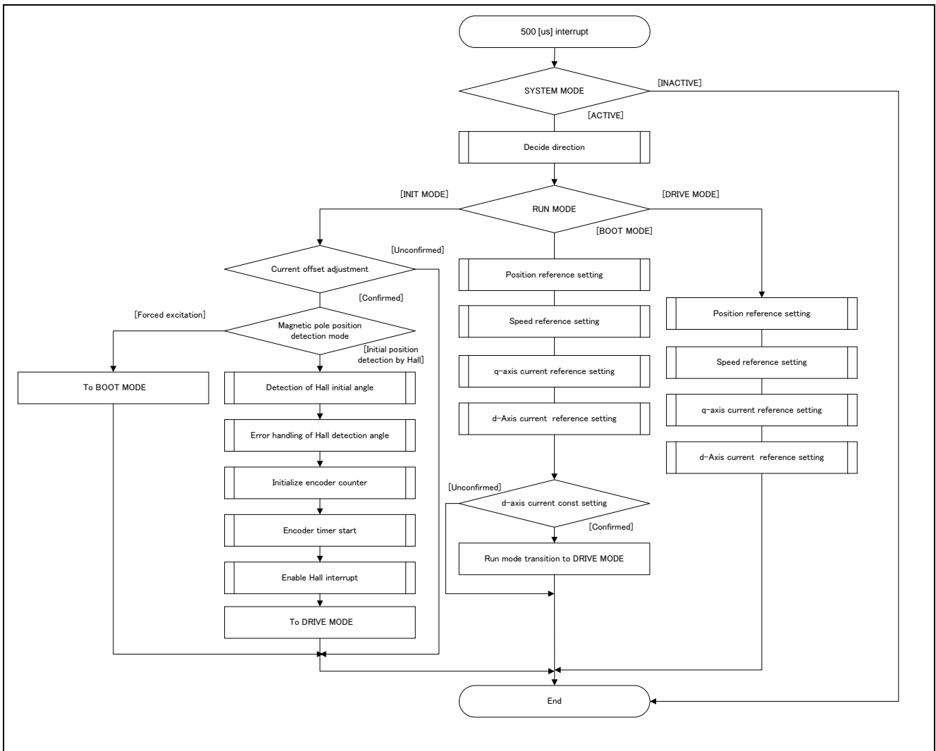
Figure 3-11 500 [μs] Interrupt Handling
