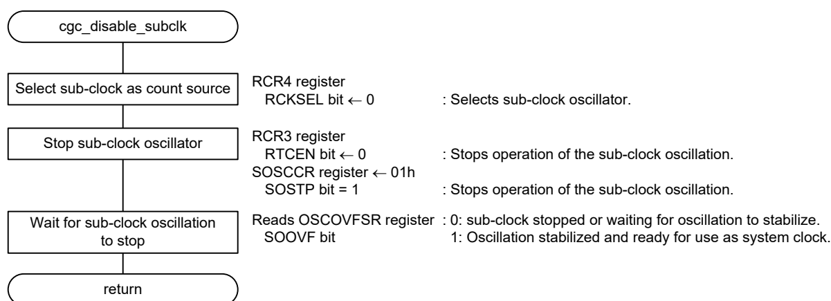
Figure 3.14 Sub-clock Disable
