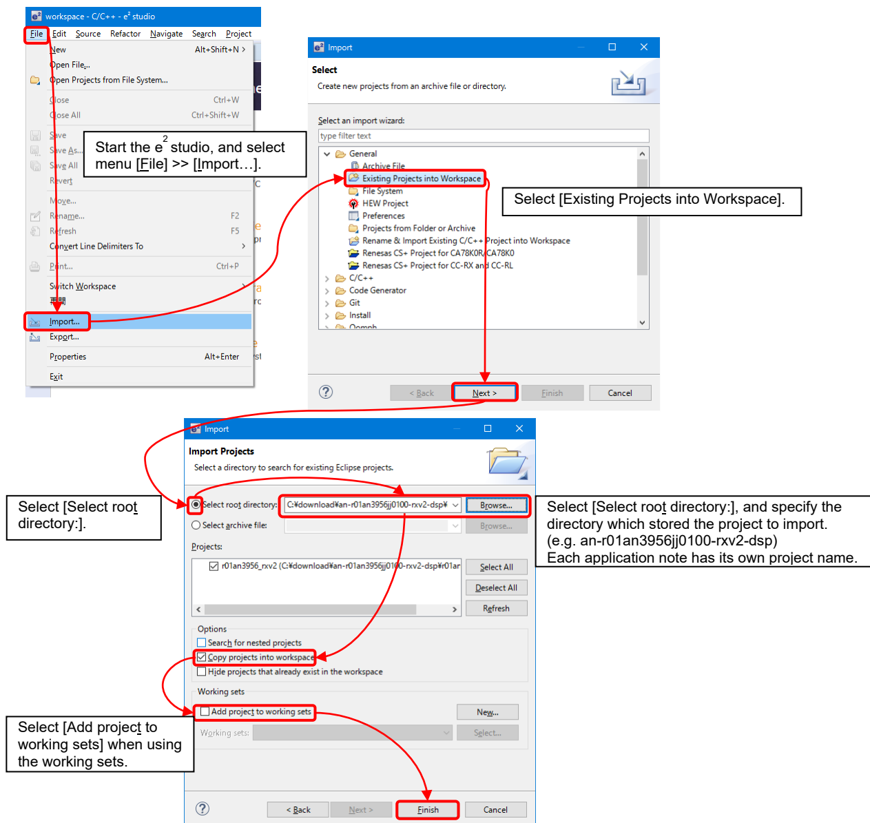
Figure 4.1 Importing a Project into e 2 studio
