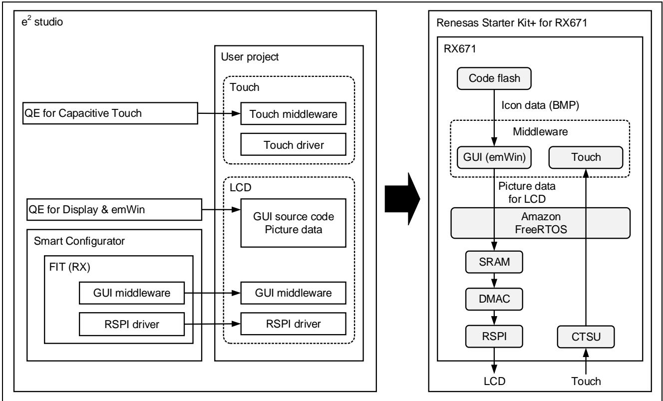
Figure 1-2 Software configuration
