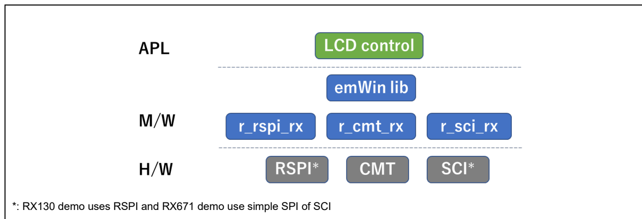
Figure 4-1 Software Hierarchy
