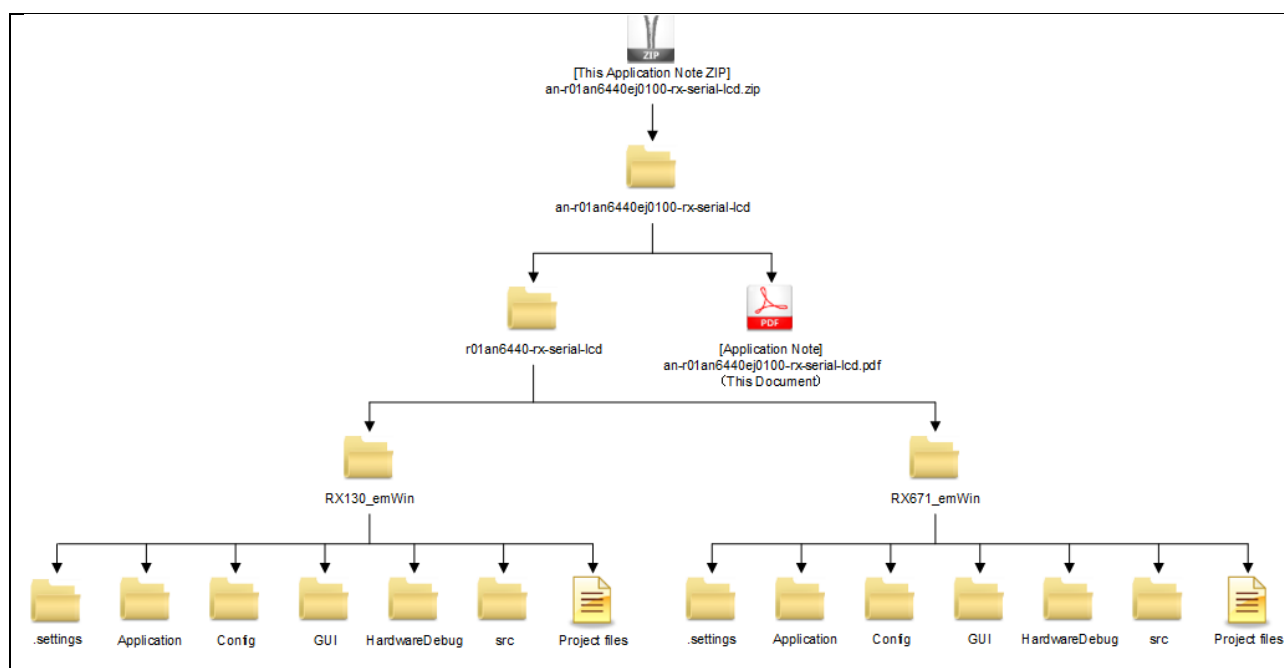
Figure 1-2 Project Structure
