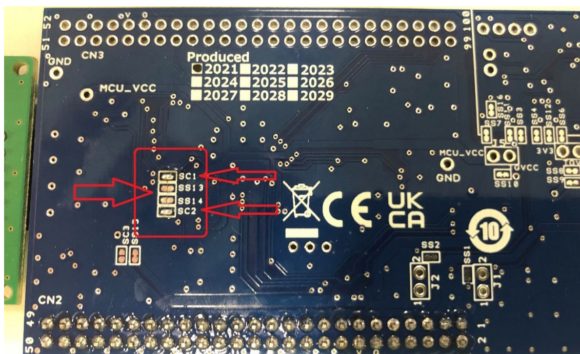
Figure 2-2 RX671 Target Board Modification
