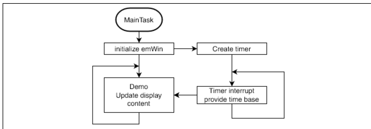
Figure 4-1 Flowchart
