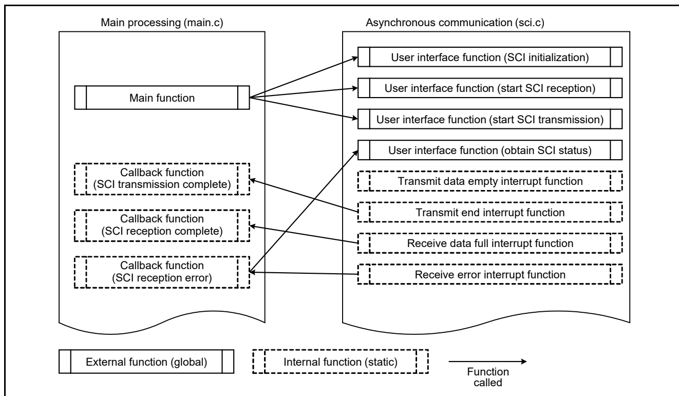
Figure 5.1 Software Configuration
