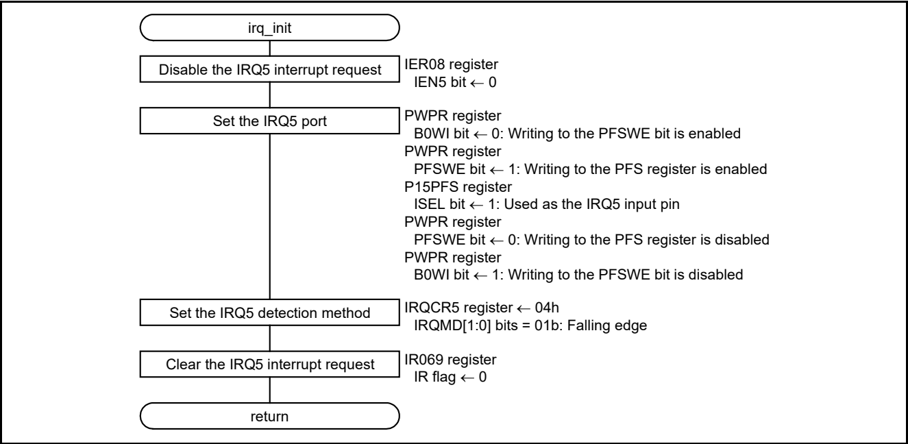
Figure 5.12 IRQ Initialization
