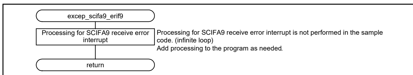
Figure 5.18 SCIFA9 Receive Error Interrupt Handling
