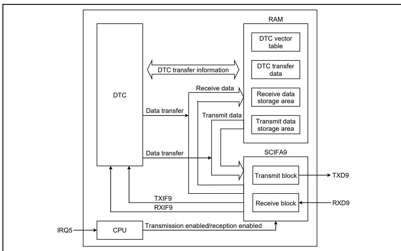
Figure 1.1 Block Diagram
