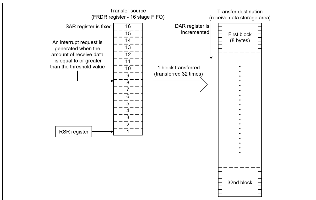
Figure 5.2 Overview of Data Reception
