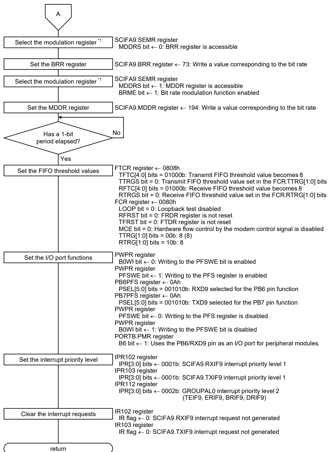
Figure 5.10 SCIFA9 Initialization (2/2)
