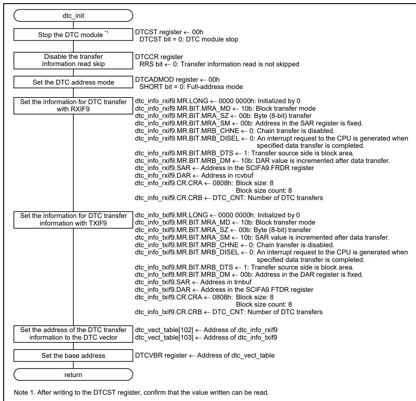
Figure 5.11 DTC Initialization
