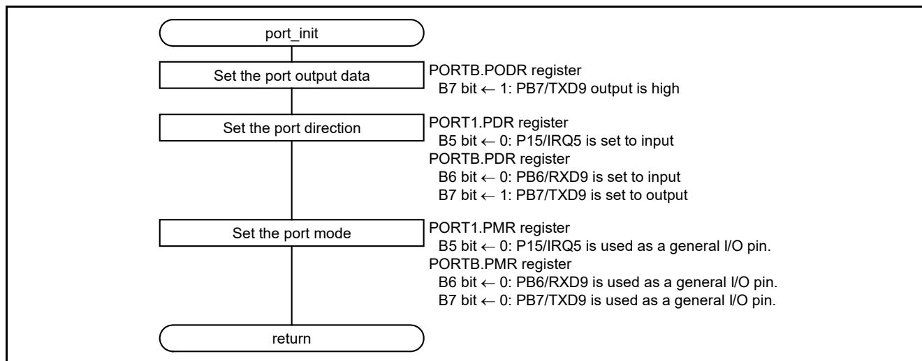
Figure 5.7 Port Initialization
