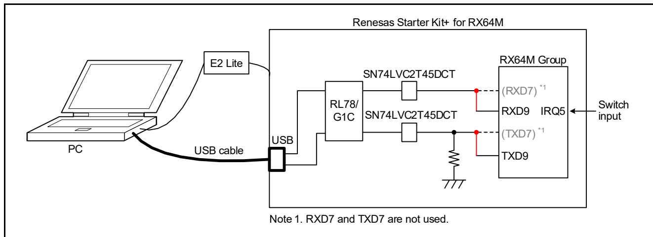
Figure 4.1 Connection Example
