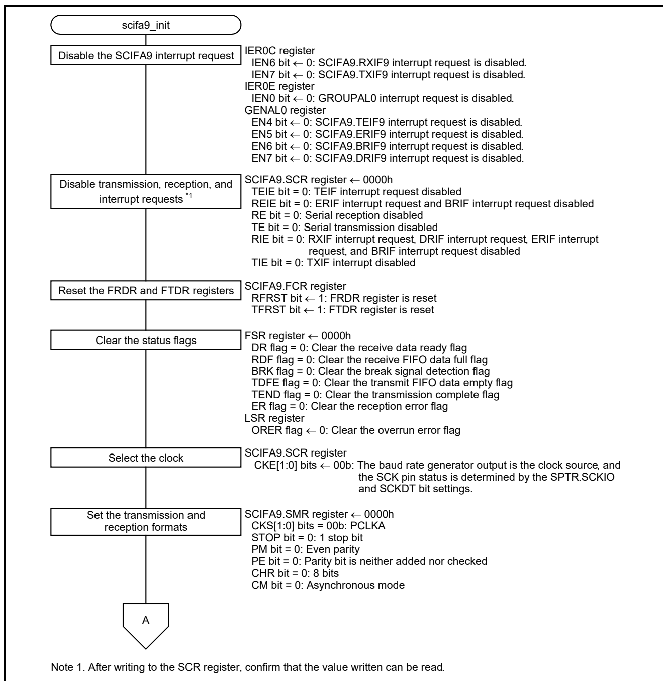
Figure 5.9 SCIFA9 Initialization (1/2)
