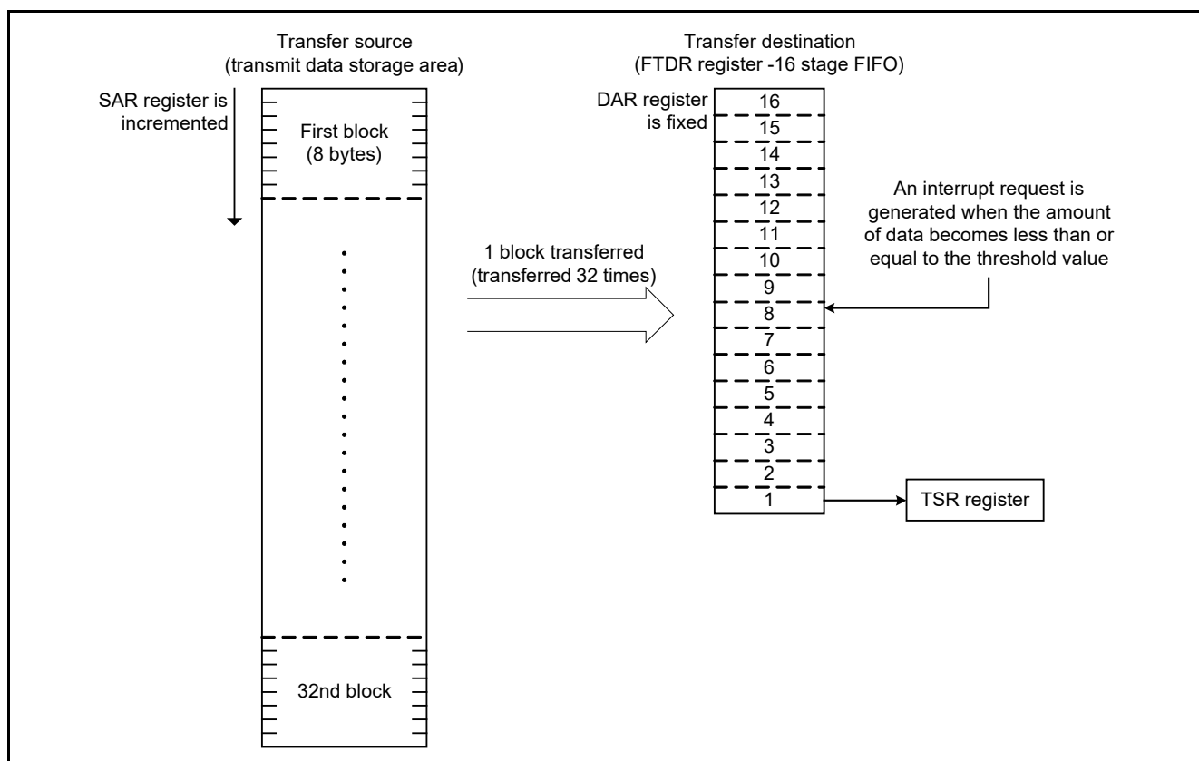
Figure 5.1 Overview of Data Transmission
