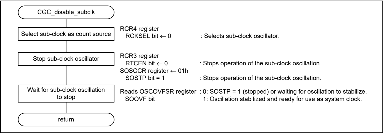
Figure 3.11 Sub-clock Disable
