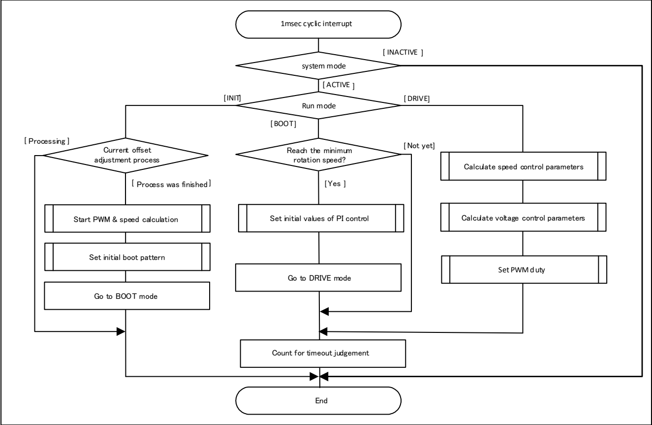
Figure 3-9 1 [ms] Interrupt Handling
