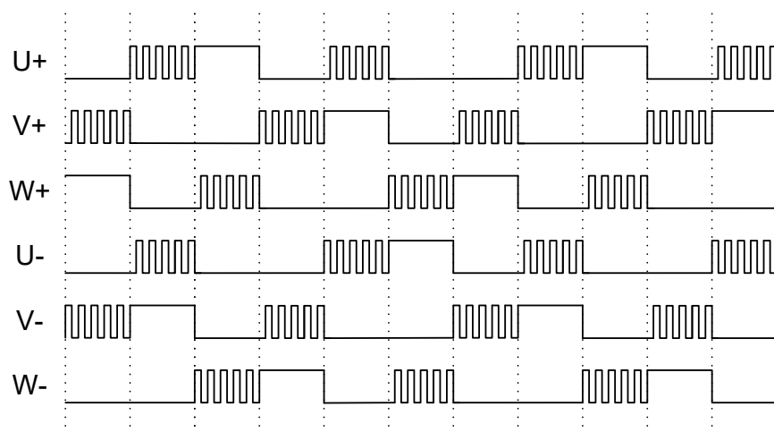
Figure 3-4 Complimentary first-60-degree Chopping
