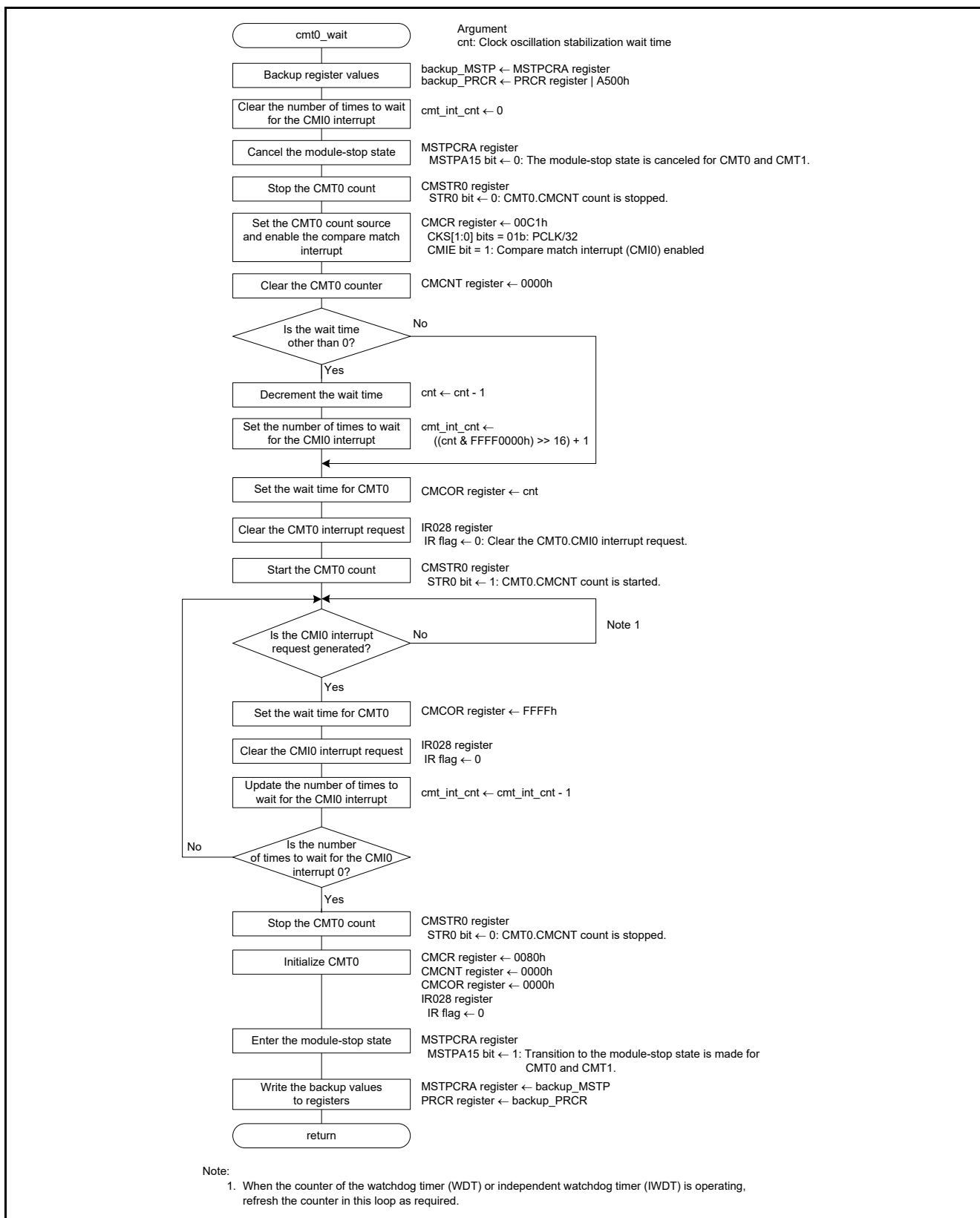
Figure 3.16 Wait Processing
