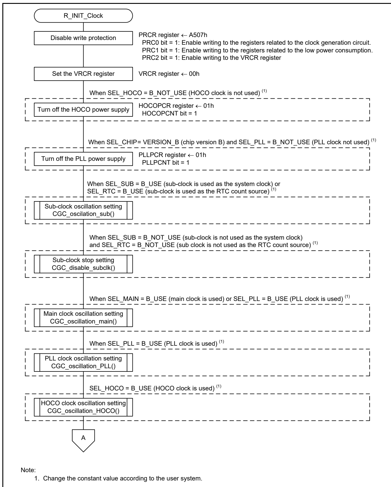
Figure 3.8 Clock Initialization (1/2)
