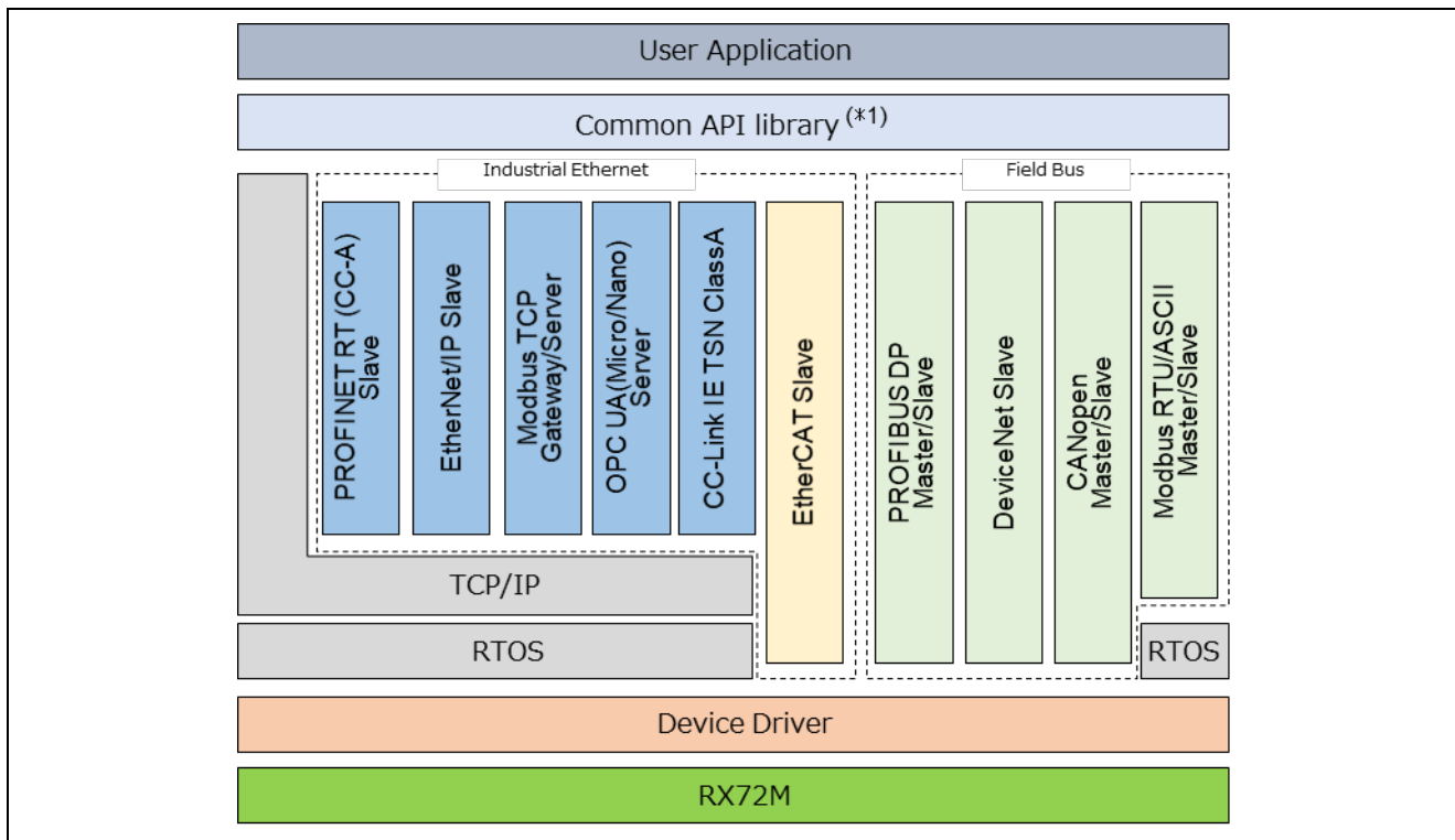
Figure 2.1 overall structure of protocol stack software for RX72M
