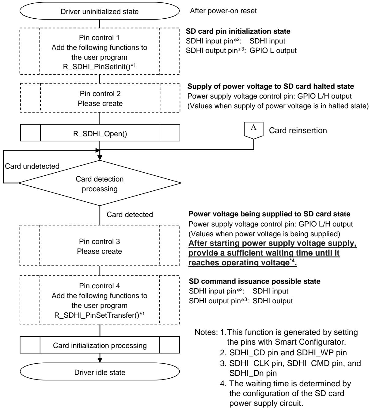
Figure 4.1 SD Card Insertion and Power-On Timing
