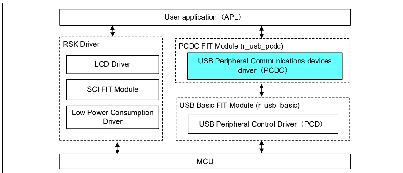
Figure 2-1 Module Configuration
