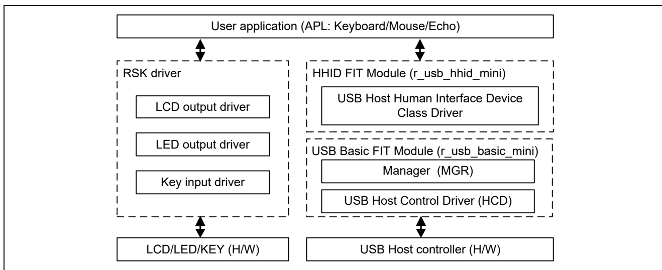
Figure 2-1 Module Configuration
