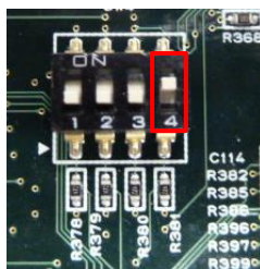
Figure 5.1 RSK RX65N Jumper Settings
