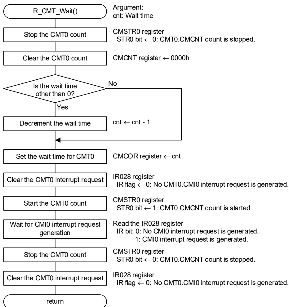
Figure 6.14 Wait Processing Using the CMT
