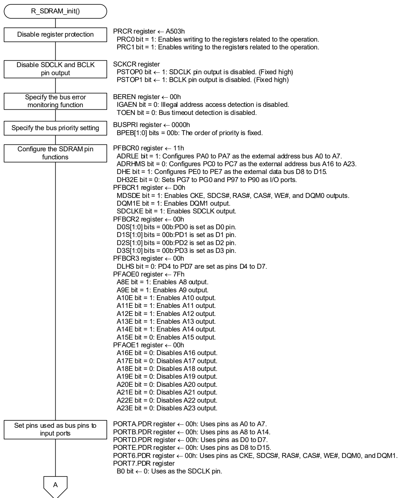
Figure 6.7 RX65N sample SDRAM Initialization (1/2)
