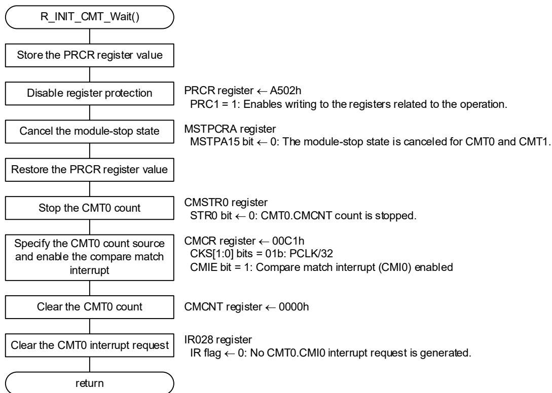
Figure 6.13 Timer Initialization for Wait Time
