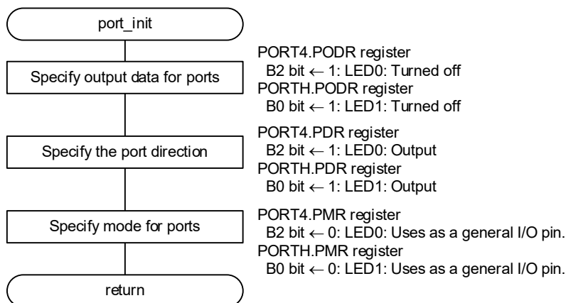
Figure 6.12 Port Initialize of RX72M projects that Smart Configurator is not used
