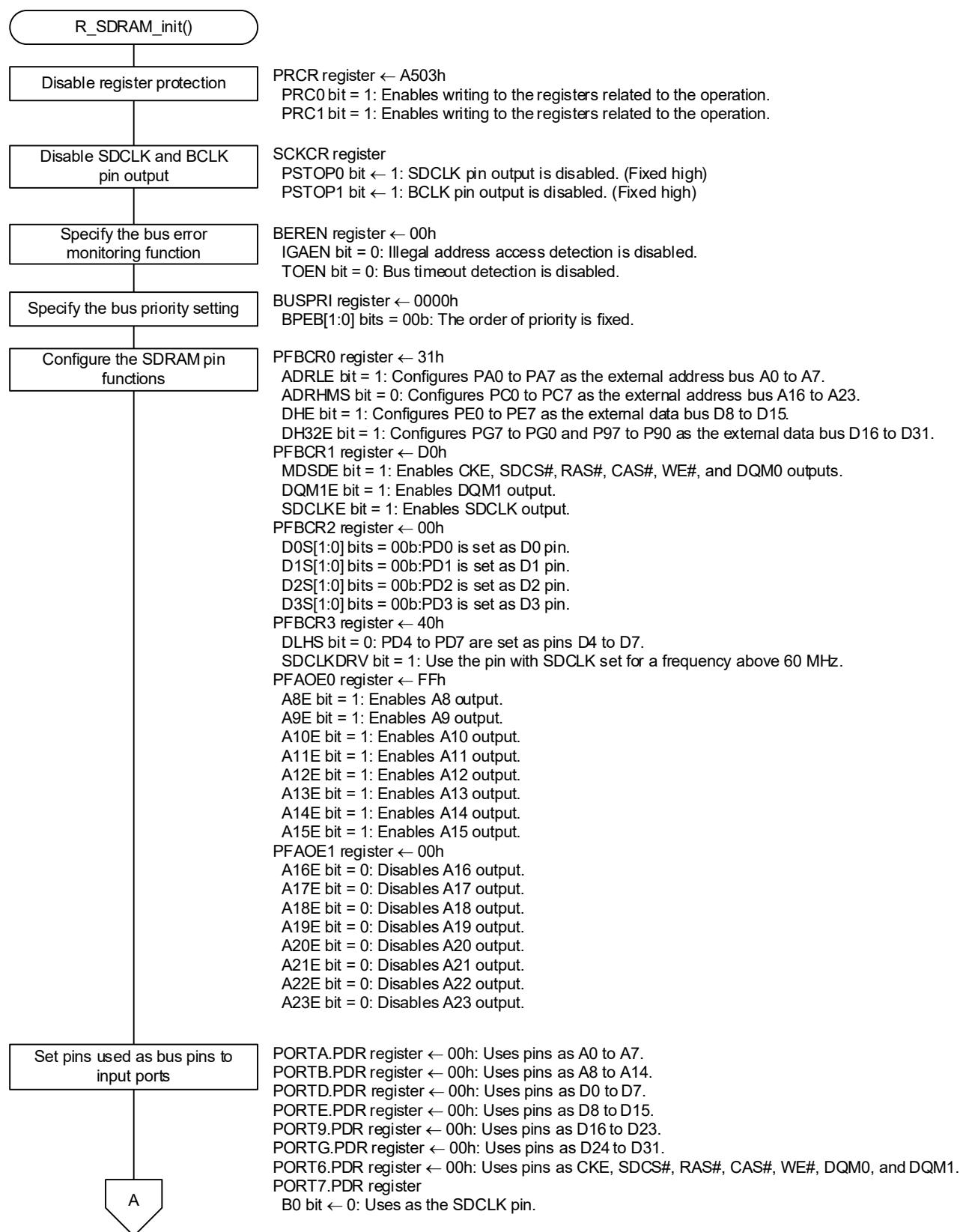
Figure 6.9 RX72M sample SDRAM Initialization (1/2)
