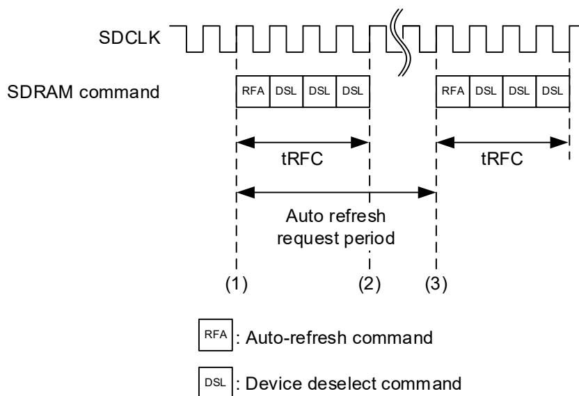
Figure 6.3 AUTO REFRESH Operating Timing
