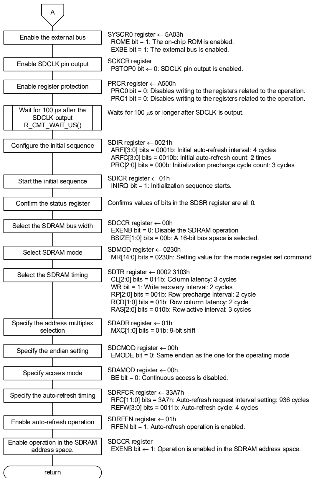
Figure 6.8 RX65N sample SDRAM Initialization (2/2)
