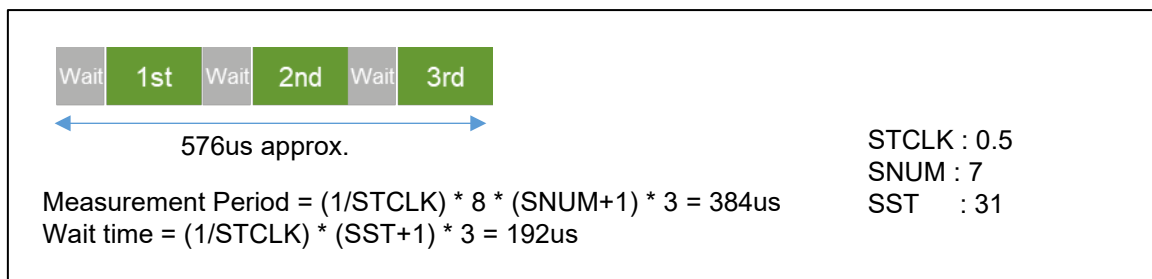
Figure 6 Self-capacitance Measurement Period (CTSUL)
