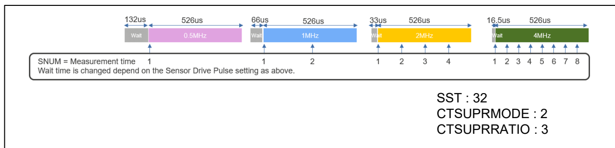
Figure 5 Self-capacitance Measurement Period (CTSUI)
