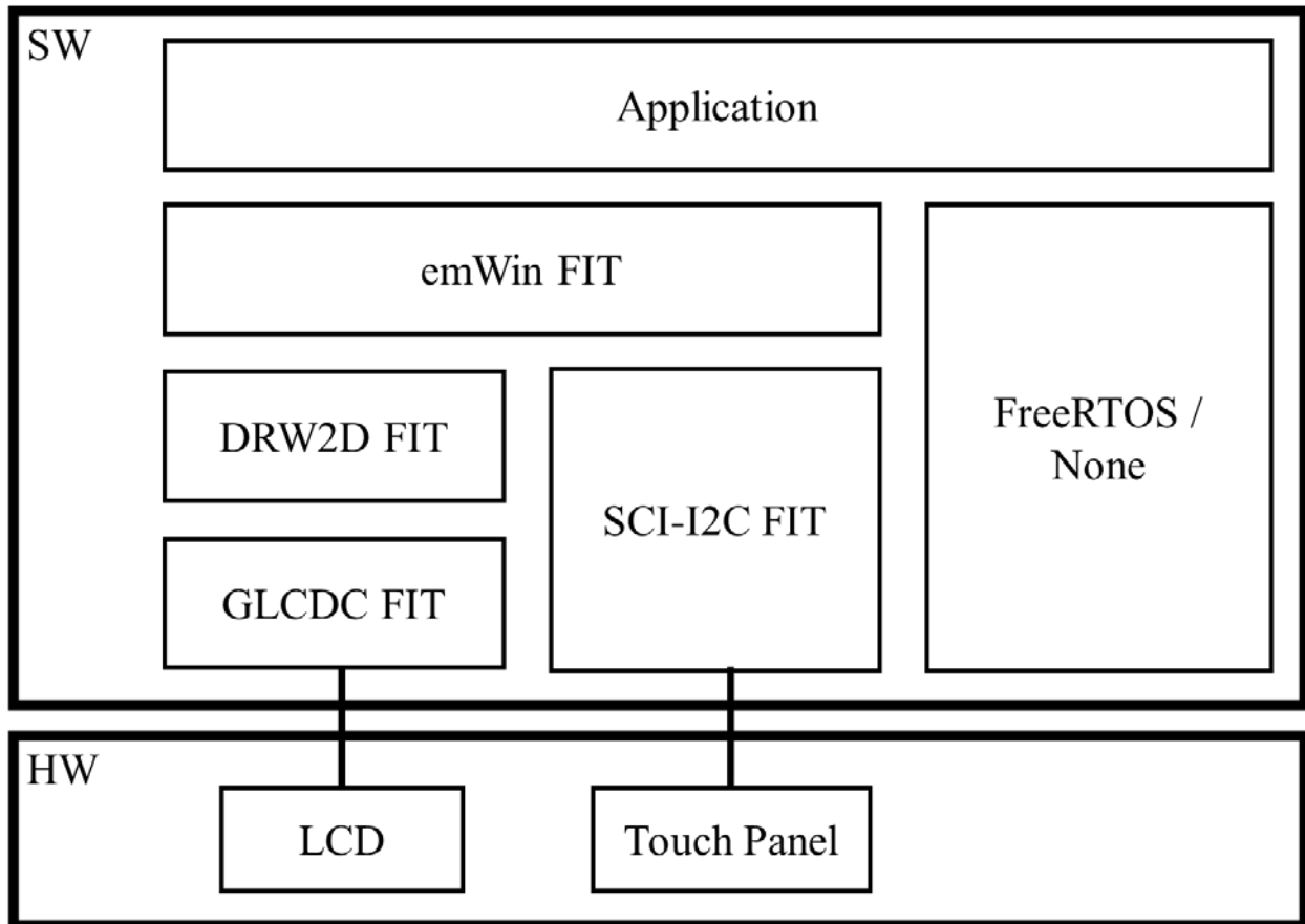
Figure 1.1 Software Configuration
