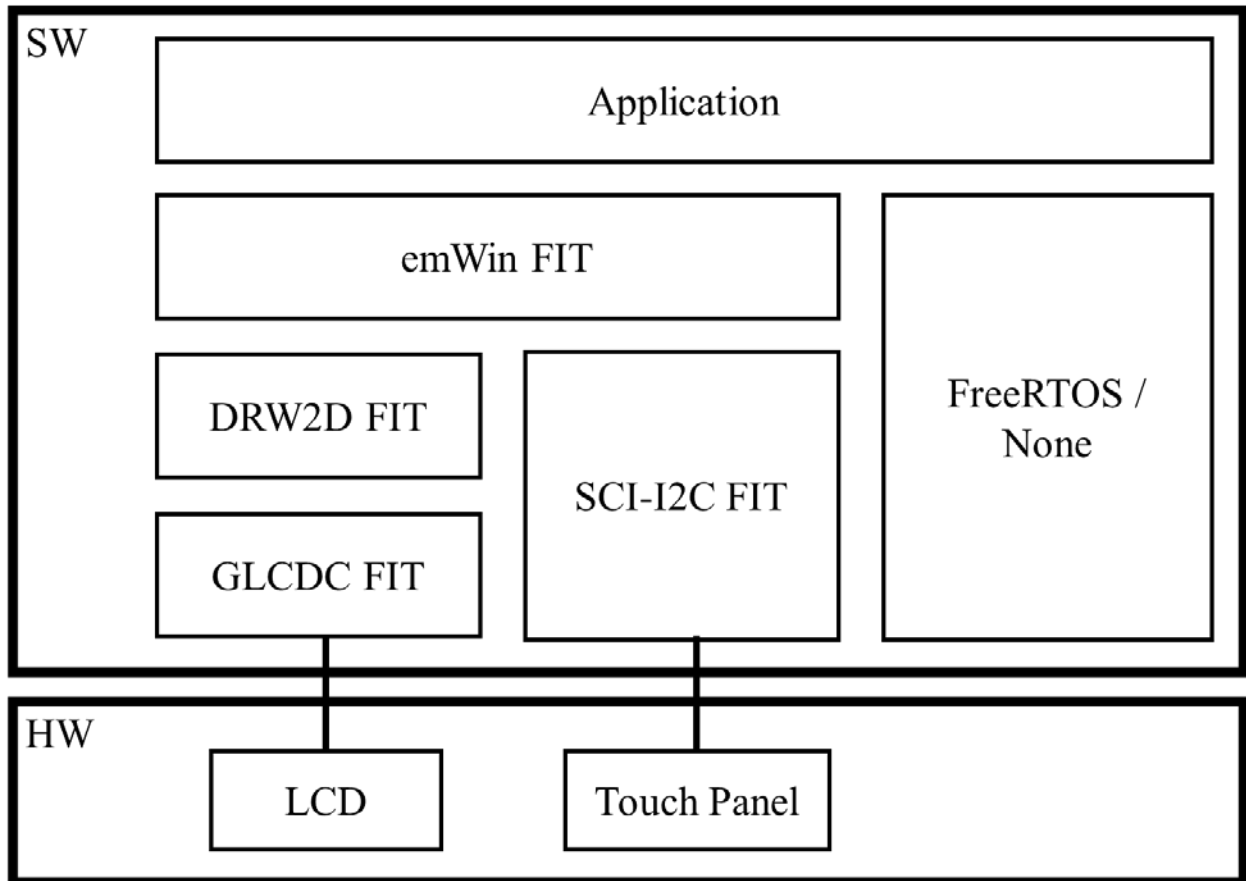
Figure 1.1 Software Configuration
