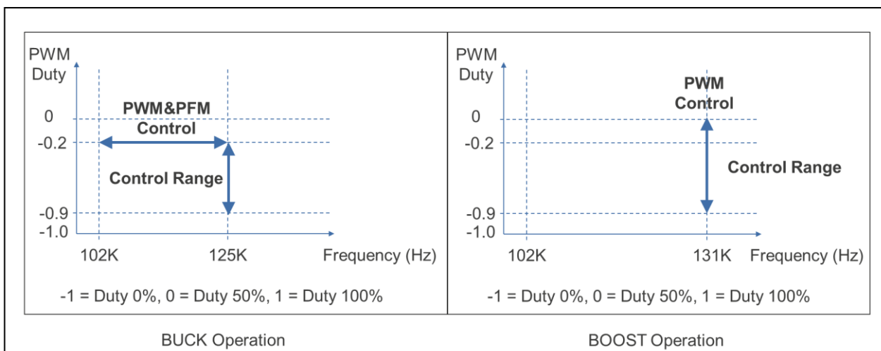
Figure 14 Relation Between Switching Frequency and Duty During BUCK/BOOST Operation
