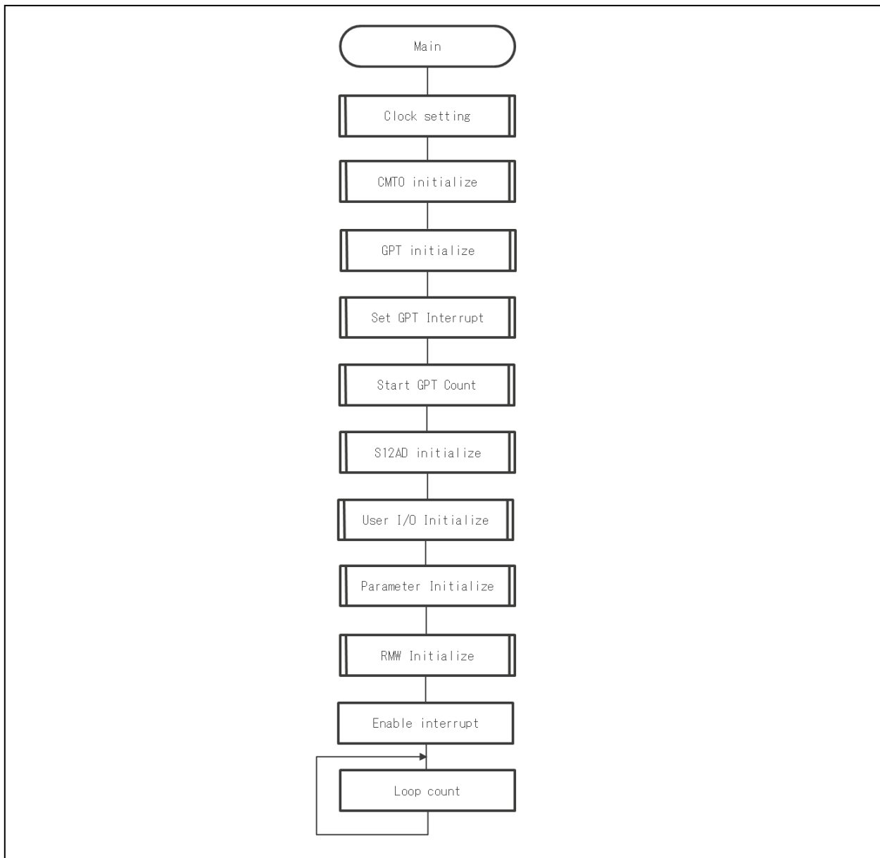
Figure 15 Main Process
