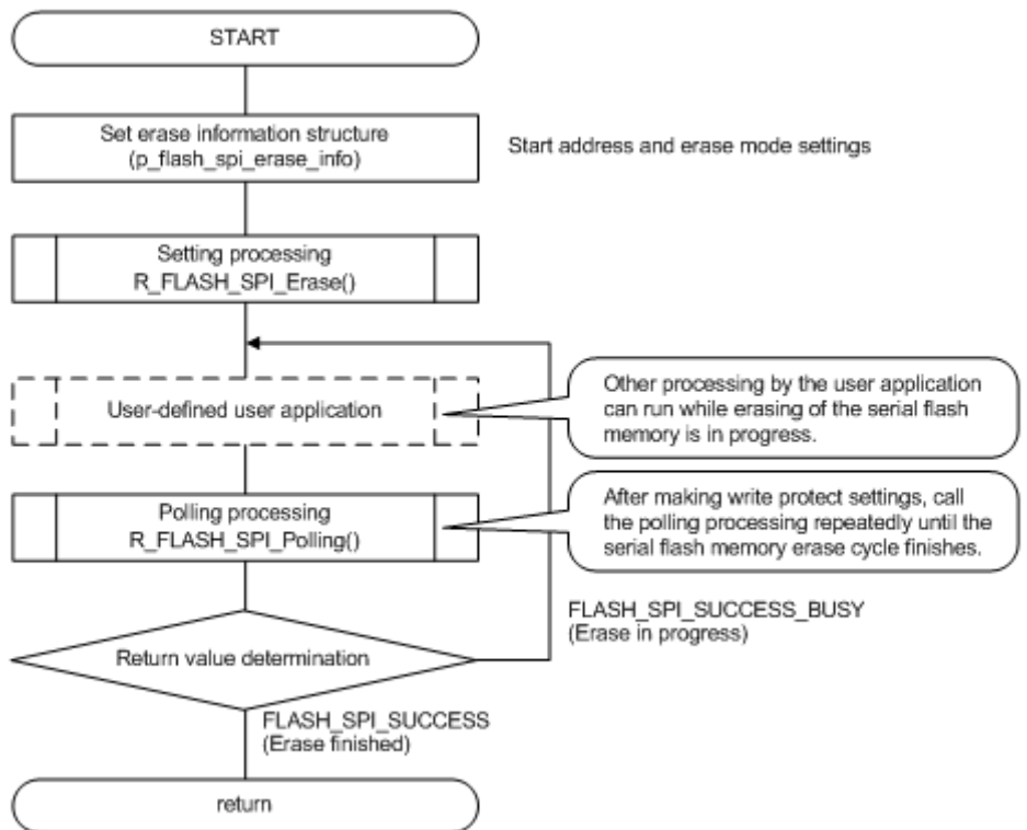
Figure 3.3 R_FLASH_SPI_Erase() Processing Example
