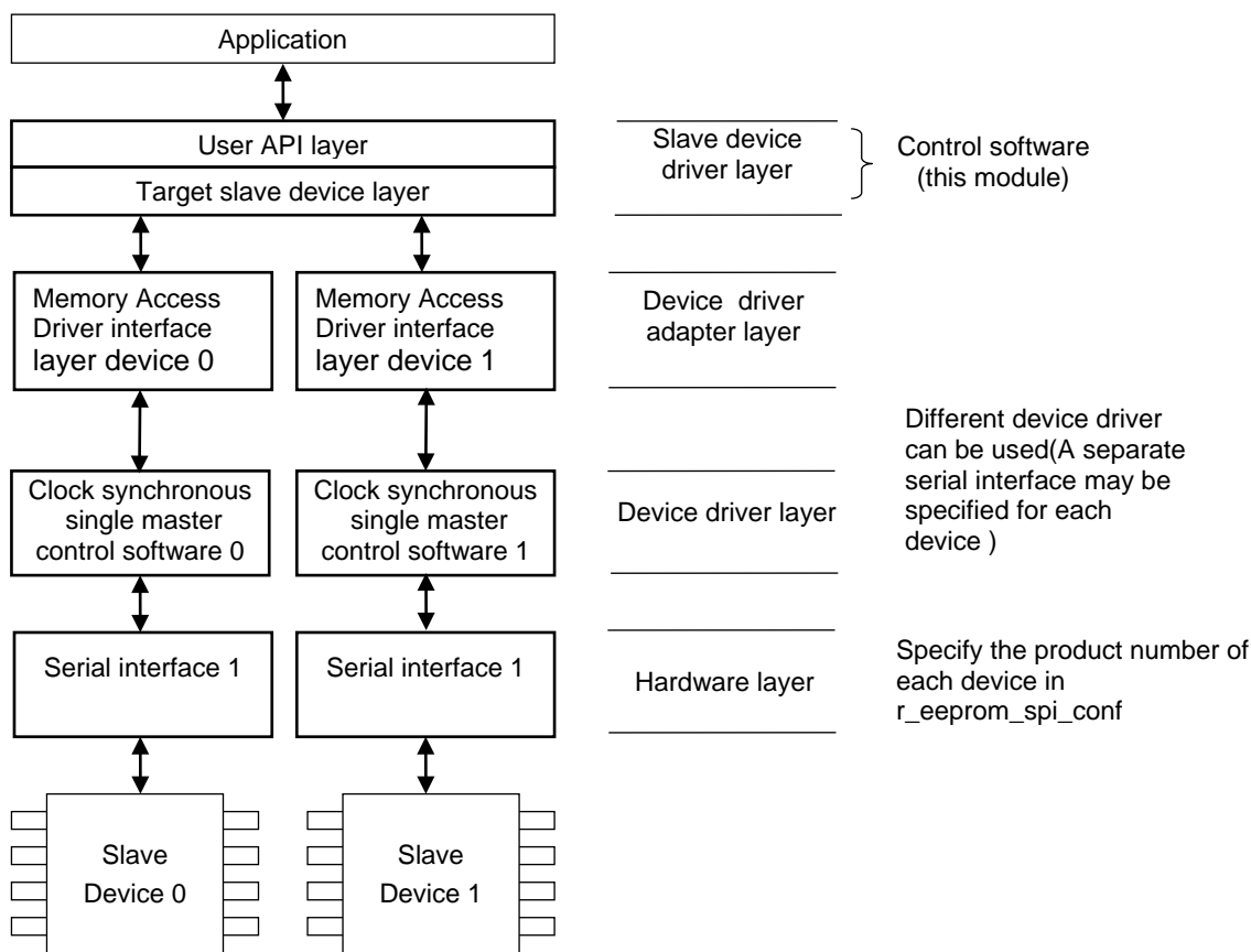
Figure 1.5 Software Configuration with Clock Synchronous Single Master Control Modules
