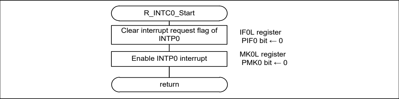
Figure 6.20 Enabling INTP0
