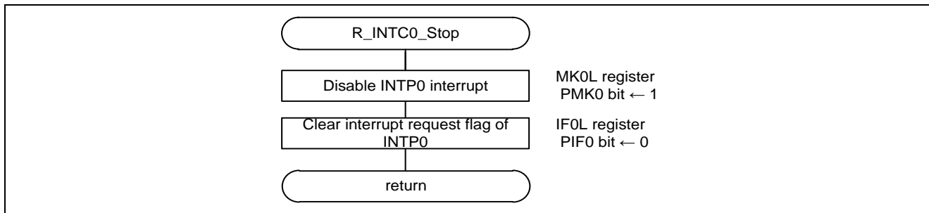
Figure 6.26 Disabling INTPO
