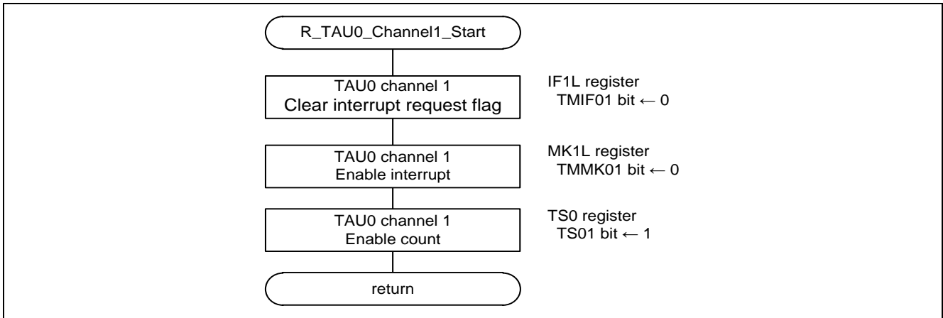
Figure 6.17 Enabling TAU01
