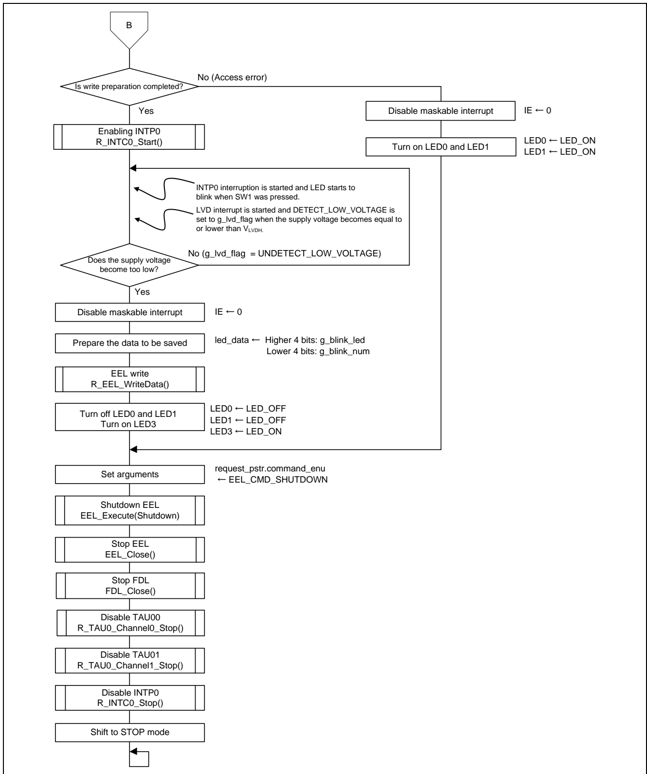
Figure 6.11 Main Processing (2/2)
