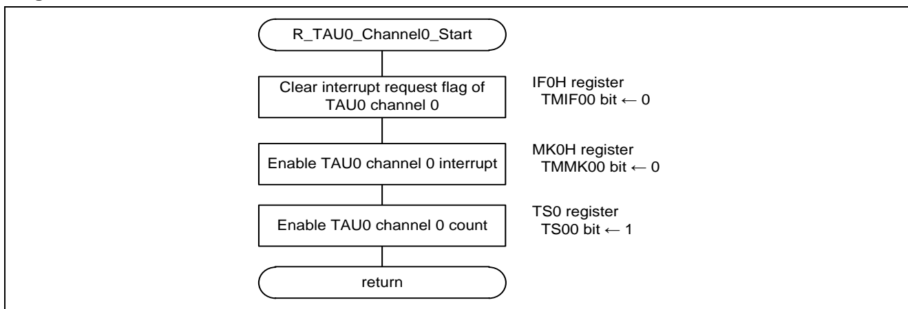
Figure 6.22 Enabling TAU00
