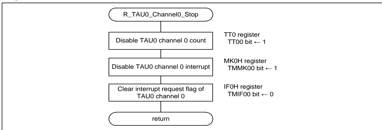
Figure 6.25 Disabling TAU00
