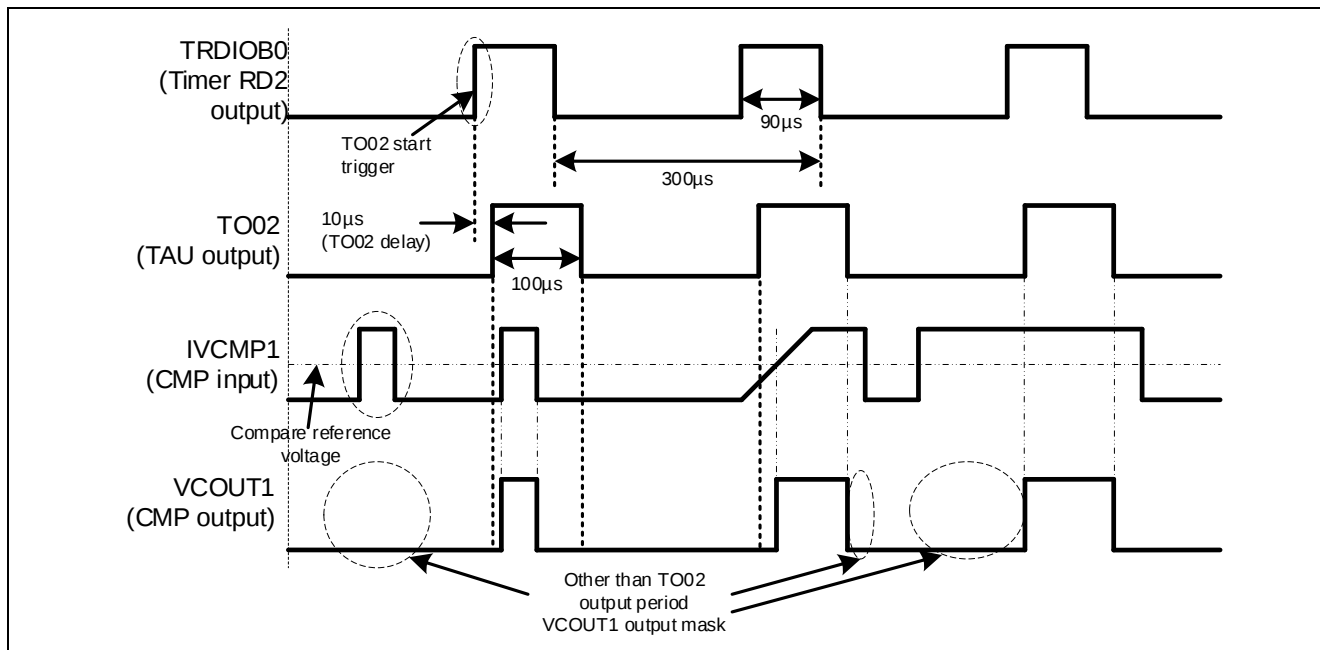
Figure 1-2 Output waveform of CMP using TIMER WINDOW Ooutput
