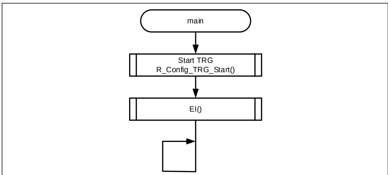
Figure 4-5 Main Process
