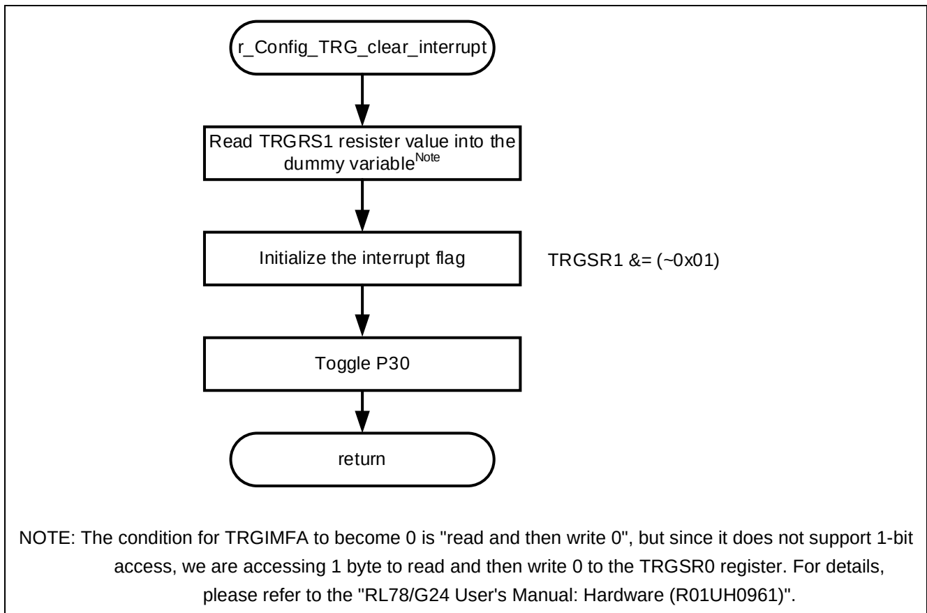
Figure 4-6 r_Config_TRG_clear_interrupt Function
