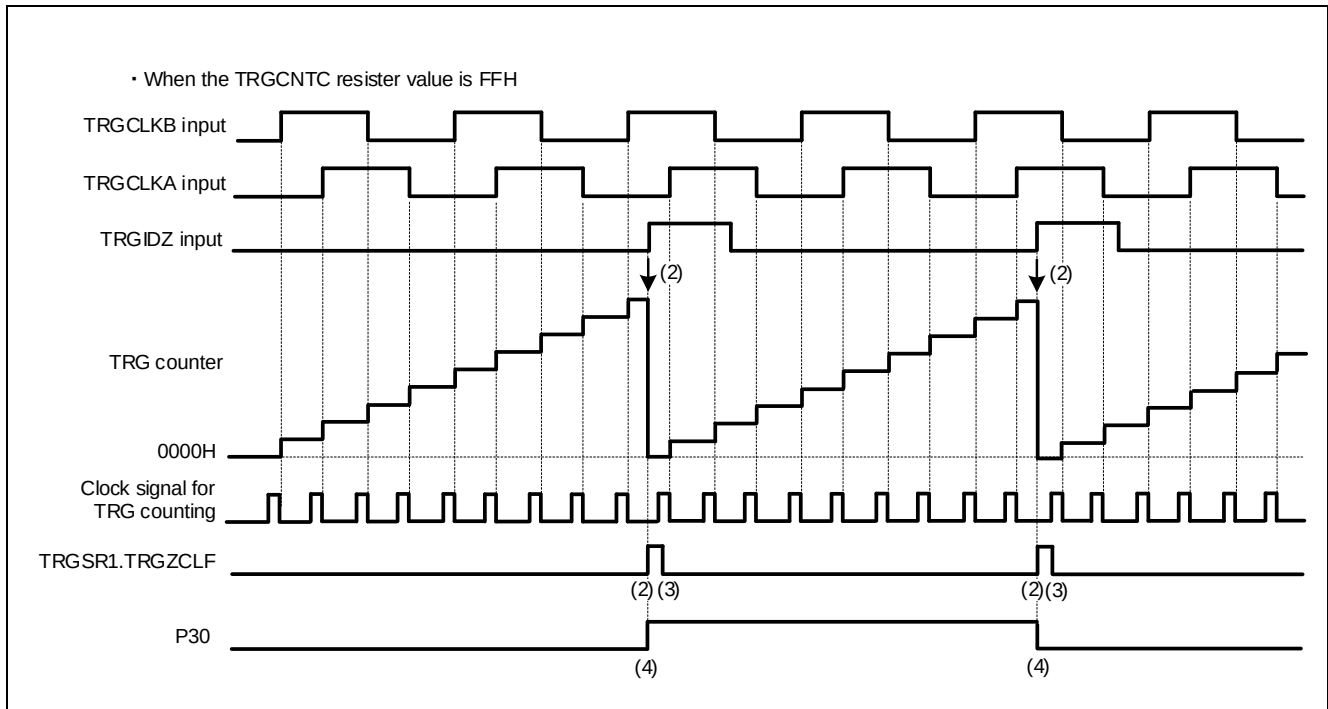
Figure 1-2 Phase Counting Mode and Port Operation
