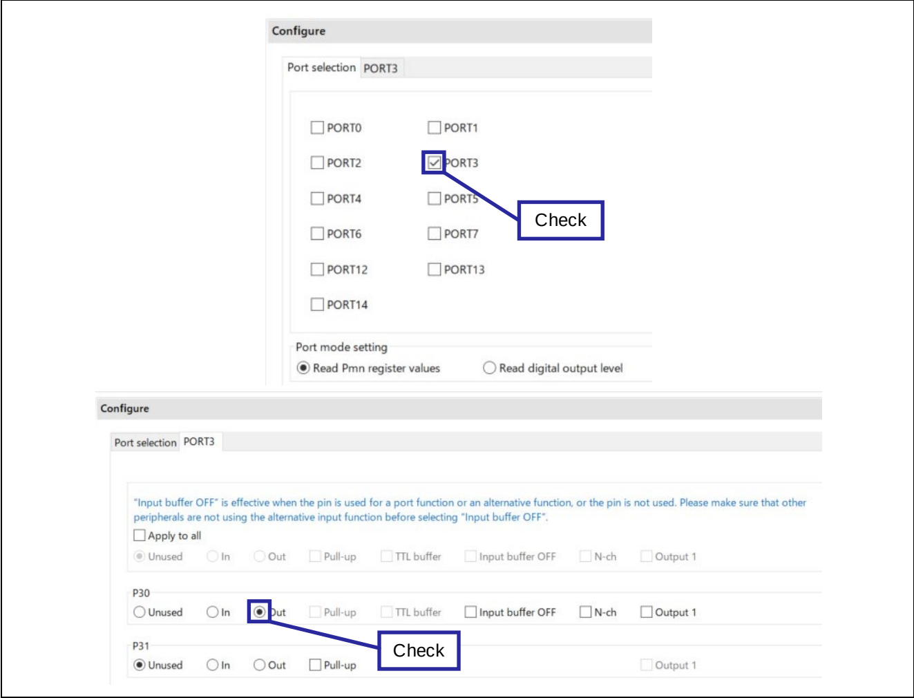
Figure 4-4 Configuration of PORT
