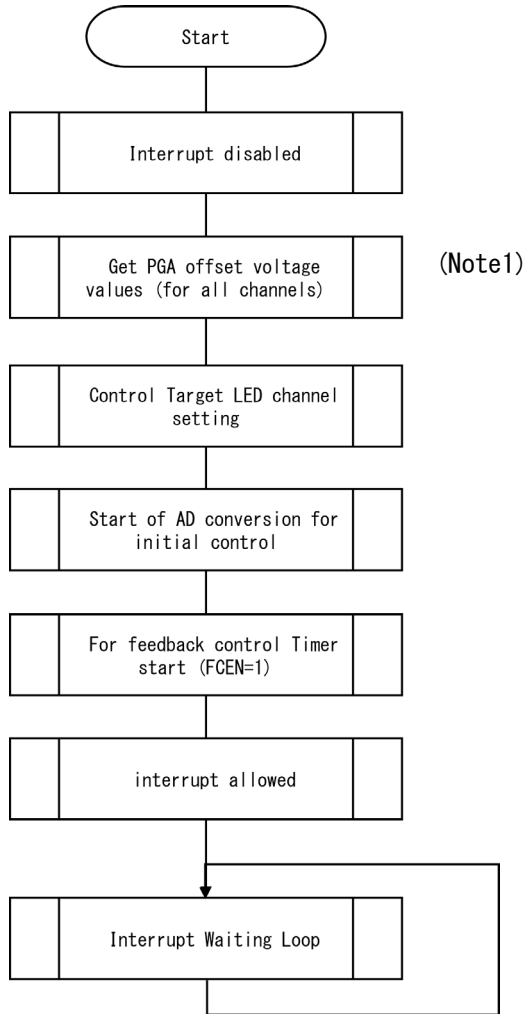
Figure 6-4 LED Control Start Processing (High-speed Operation)
