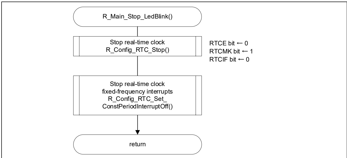
Figure 4-8 Stopping LED Blink
