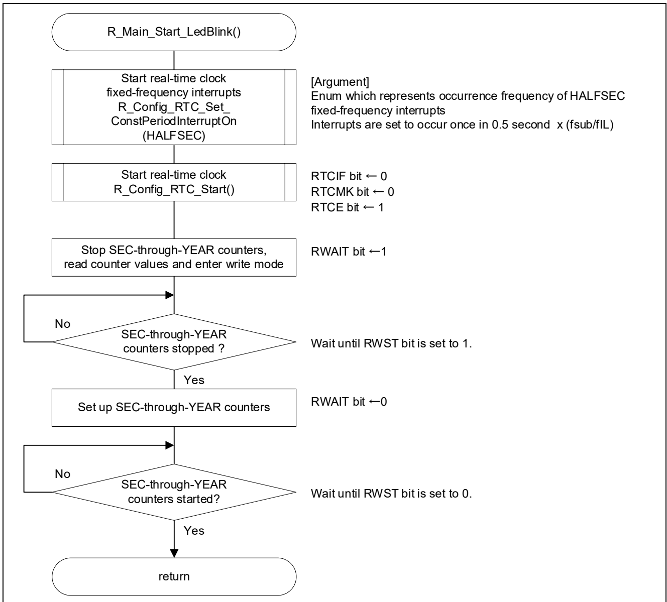
Figure 4-7 Starting LED Blink
