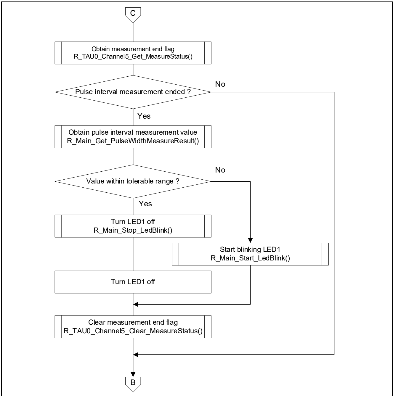
Figure 4-2 Main Processing (2/3)
