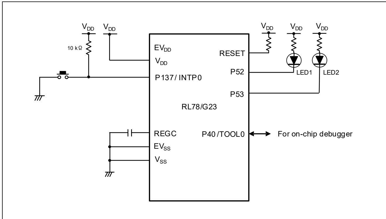
Figure 3-1 Hardware Configuration
