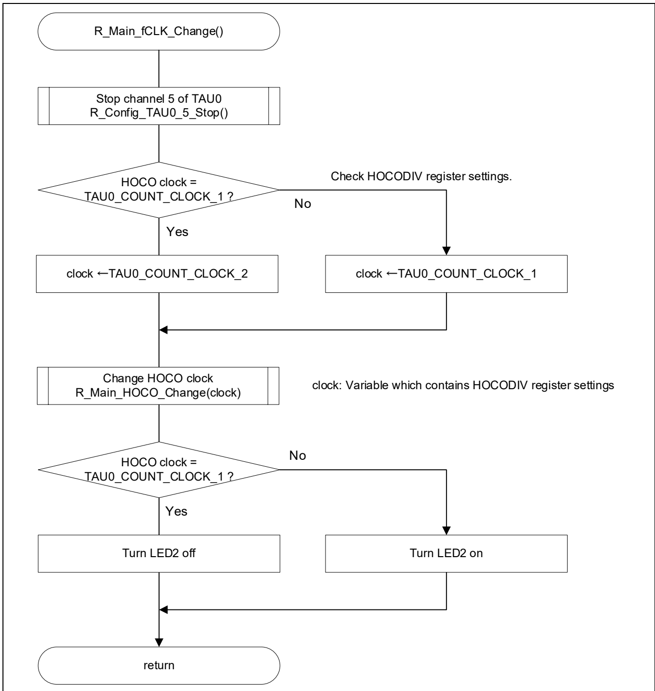
Figure 4-4 Changing Count Clock
