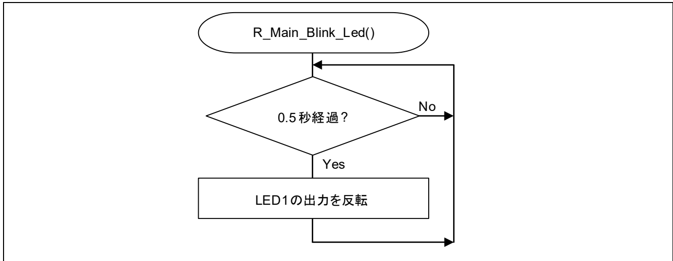
図 4 - 8 LED 点滅
