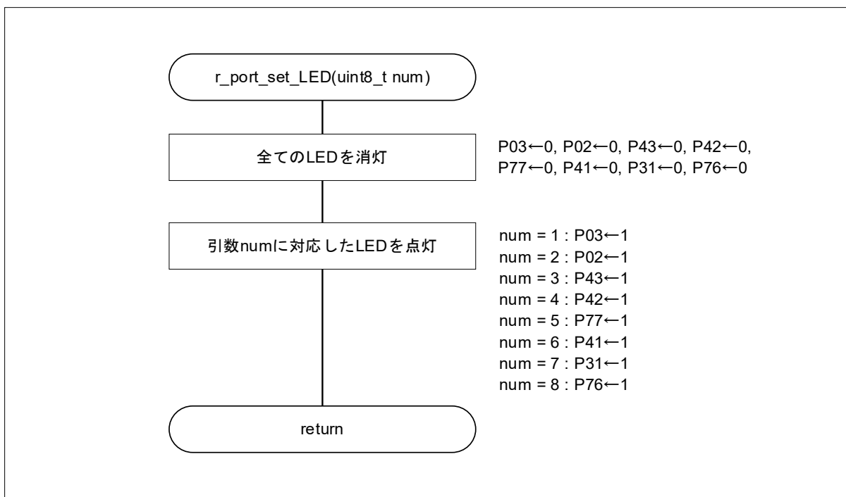
図 4-7 LED 点灯制御
