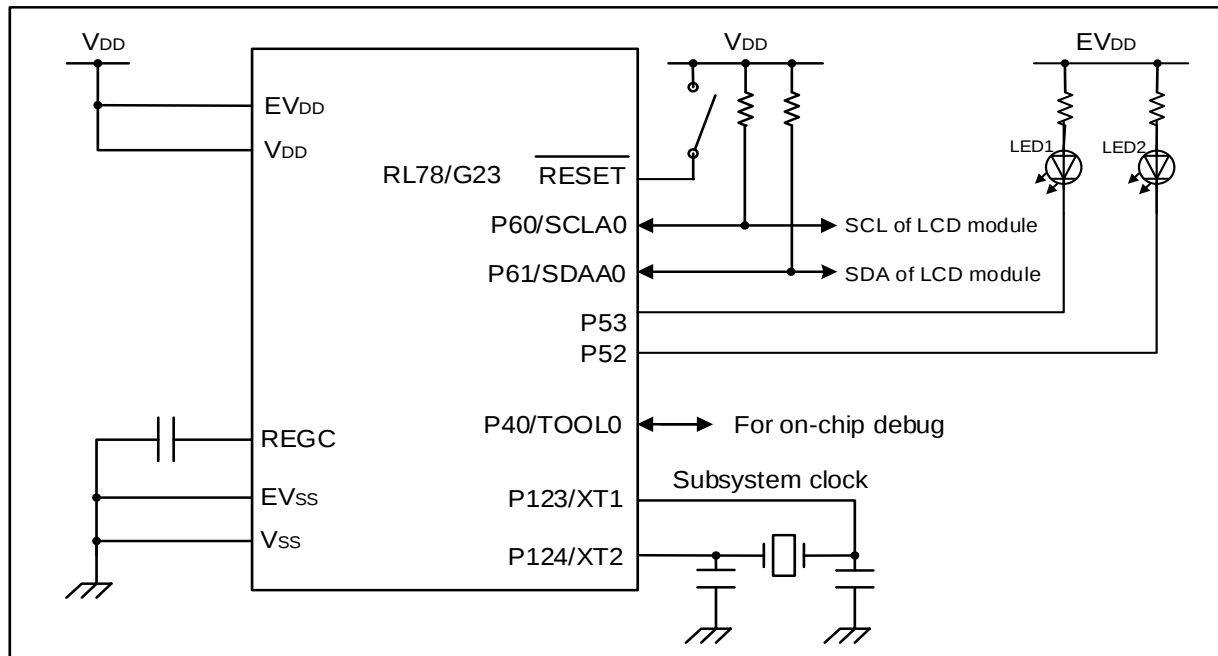
Figure 3-1 Hardware Configuration
