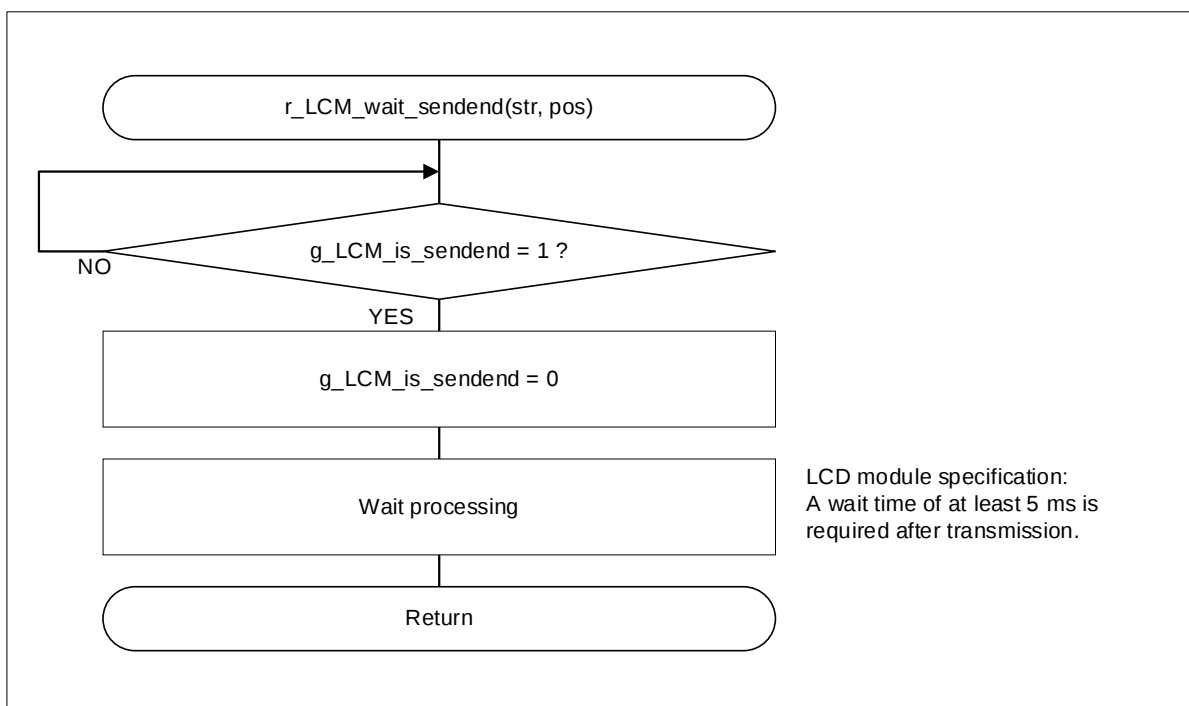
Figure 4-22 LCD Module Communication End Wait Processing
