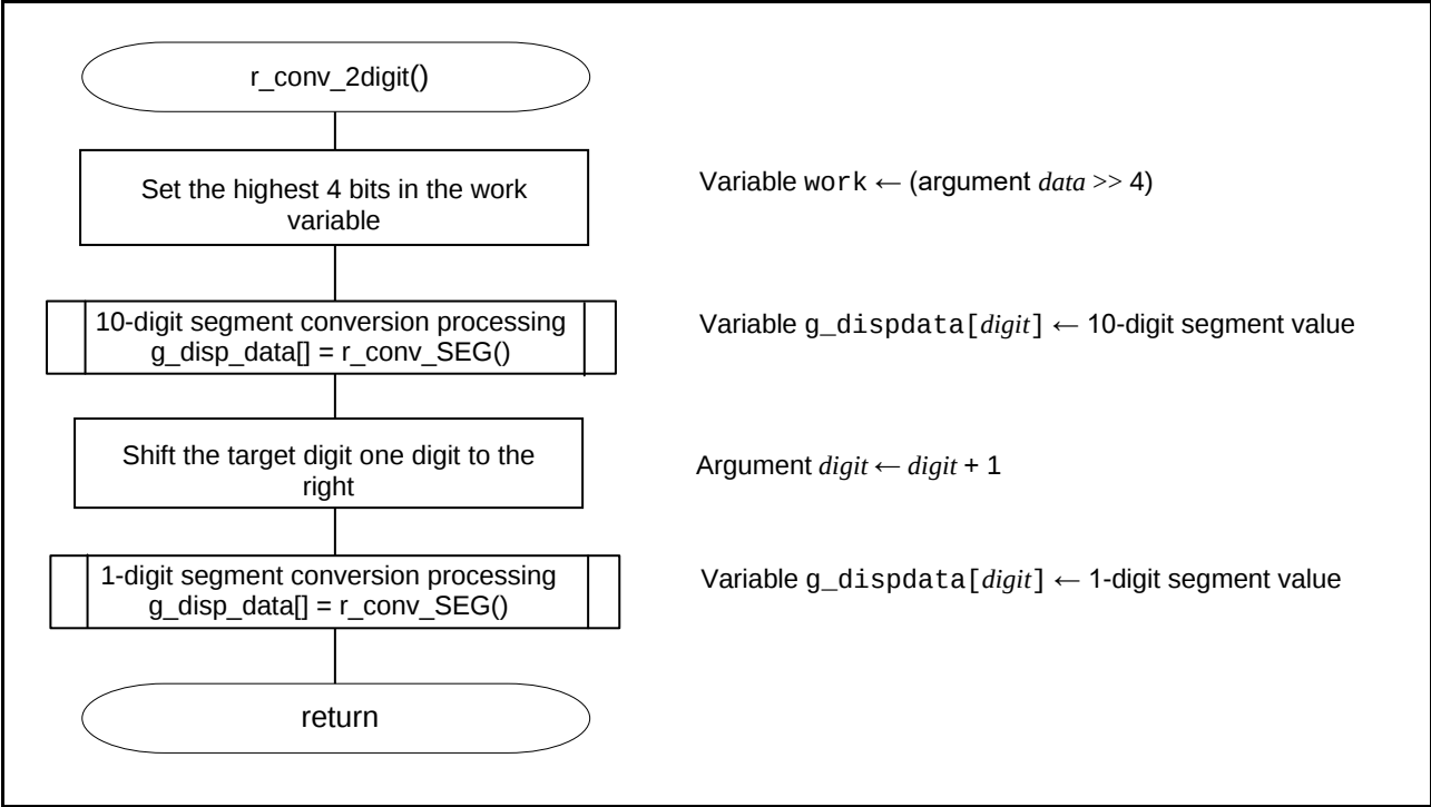
Figure 5-3 2-Digit Minute Segment Conversion Processing
