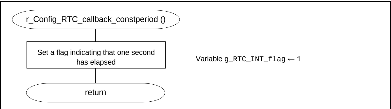
Figure 5-6 RTC Callback Processing
