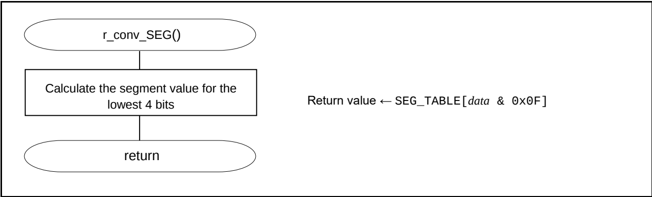
Figure 5-4 Segment Data Conversion Processing
