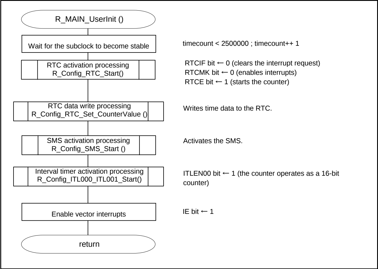
Figure 5-2 Main User Initialization Processing
