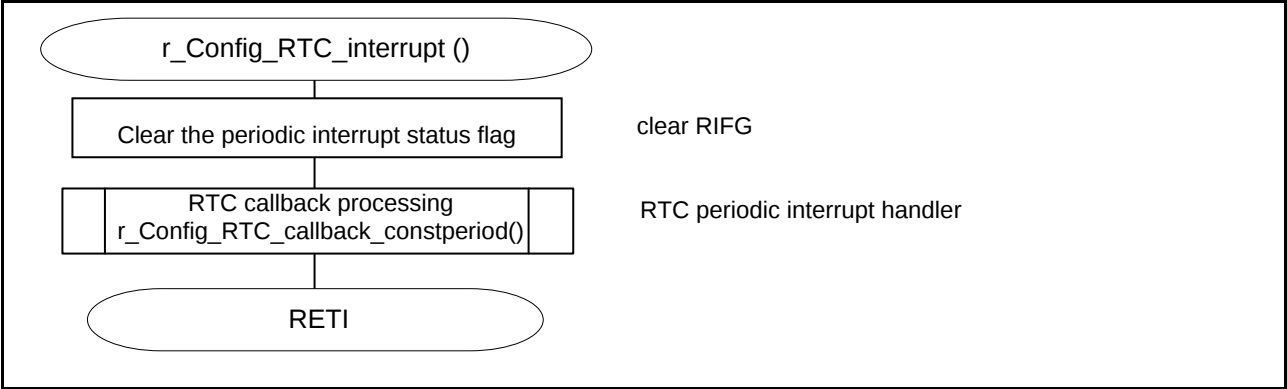
Figure 5-5 RTC 1-Second Interrupt Processing
