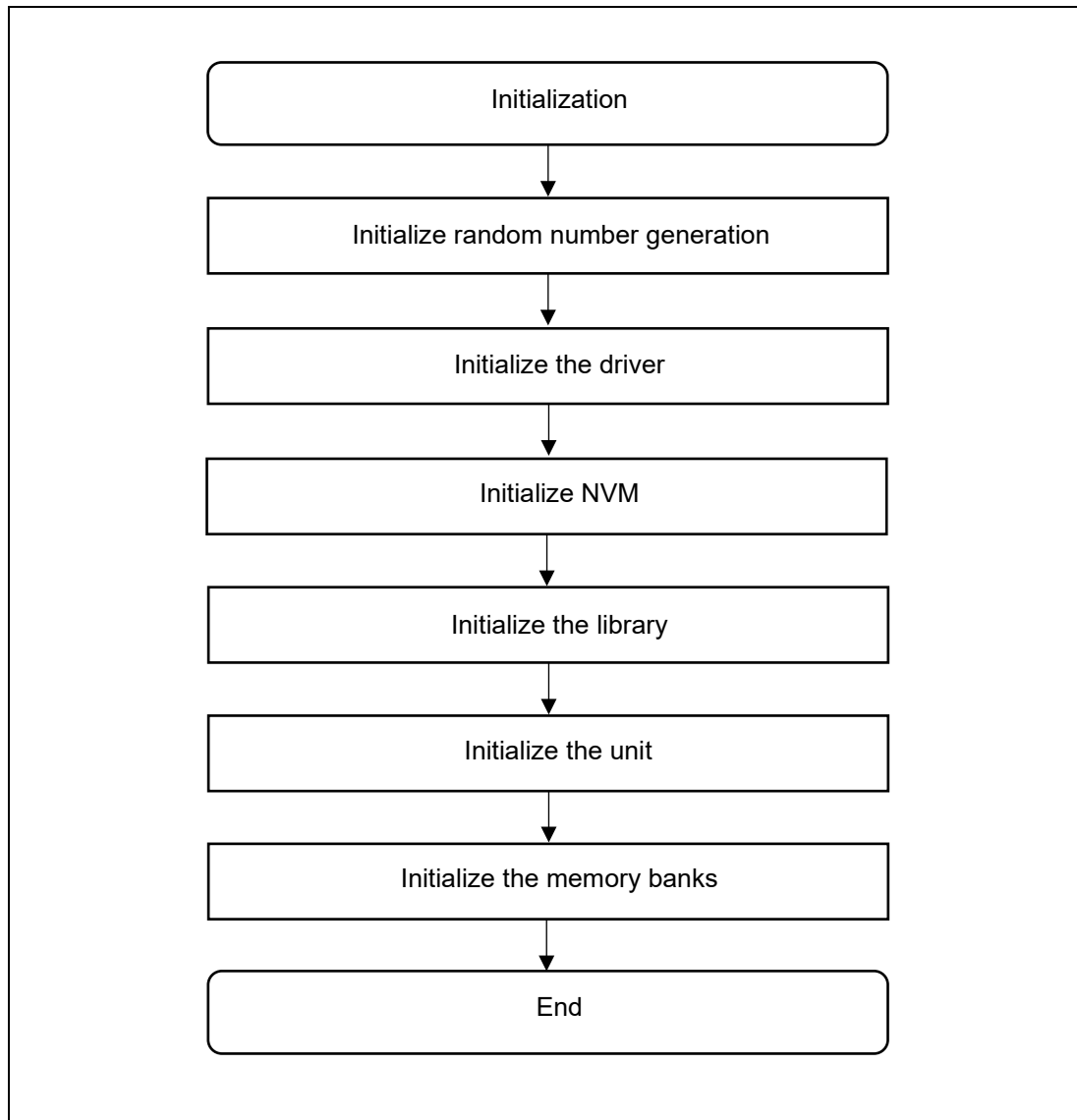
Figure 4-17 Initialization process flow diagram
