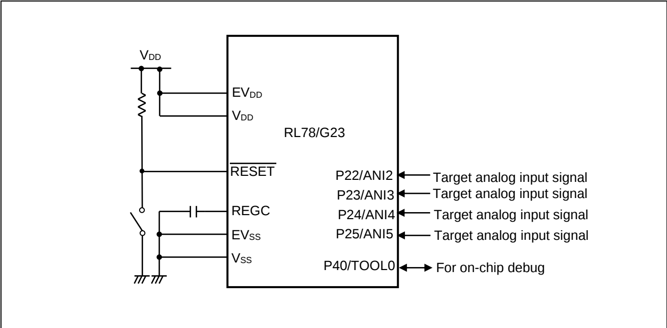
Figure 3-1 Hardware Configuration
