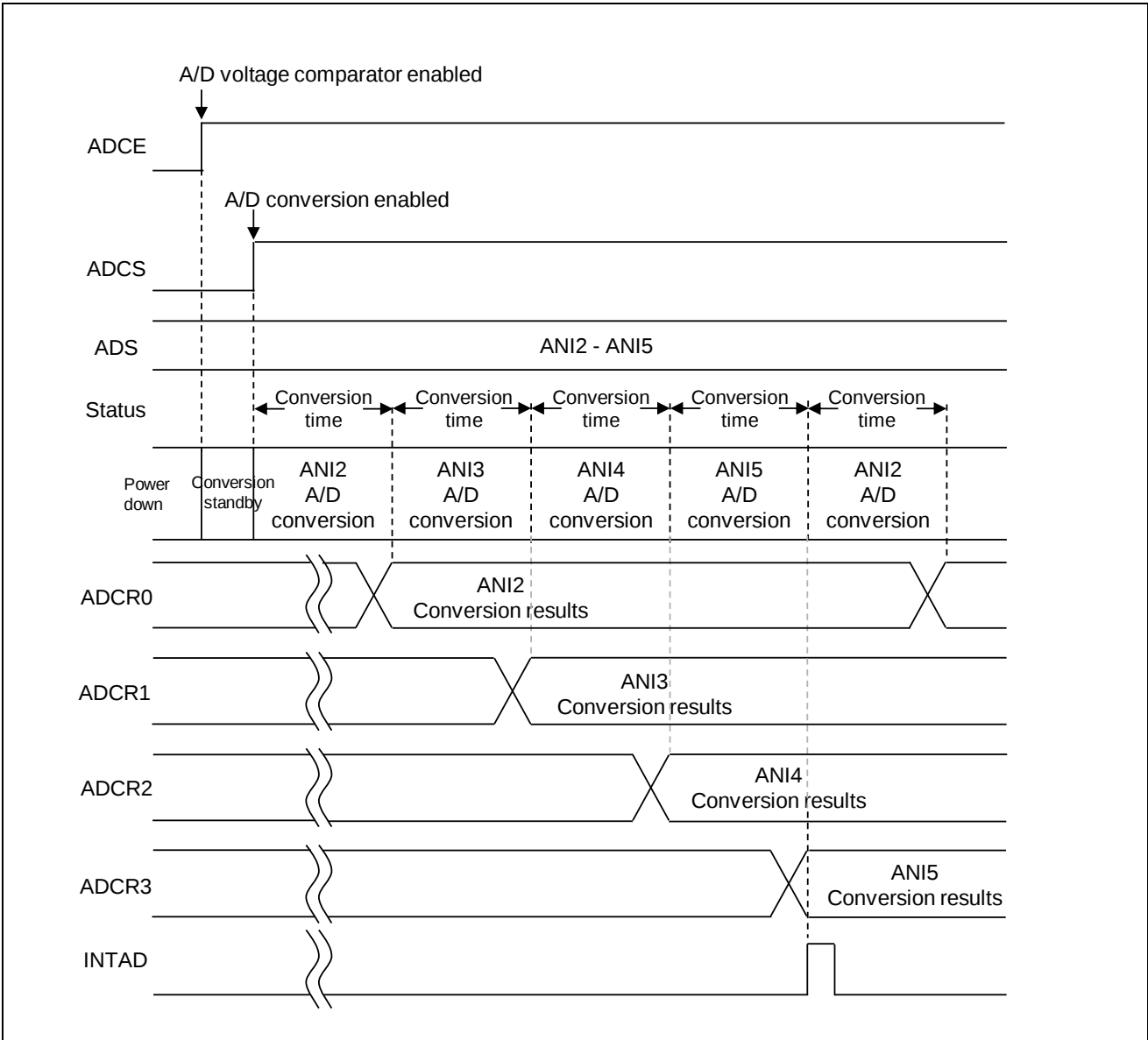
Figure 1-1 Outline of the A/D Converter Conversion Processing
