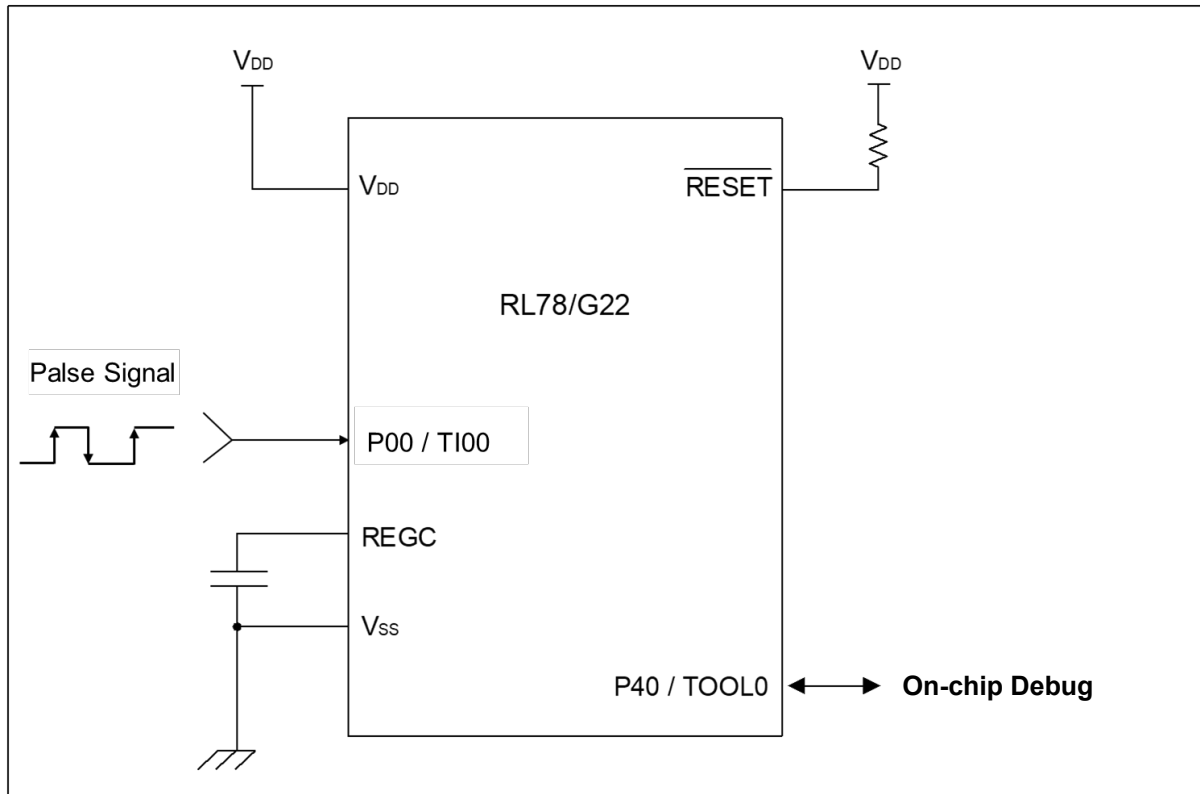
Figure 3-1 Hardware Configuration
