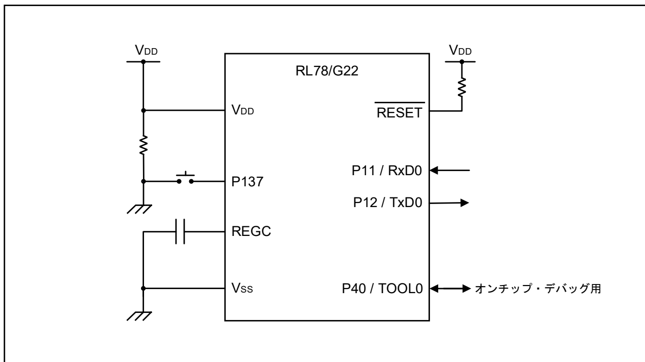
Figure 3-1 Hardware Configuration
