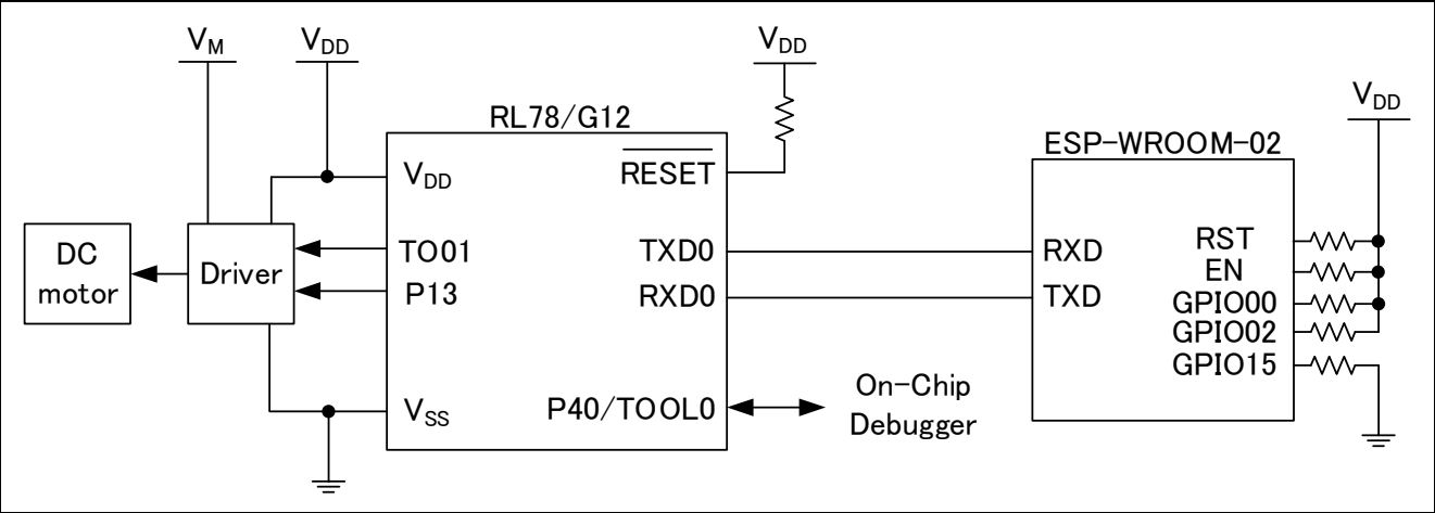
Figure 3.1 Hardware Configuration
