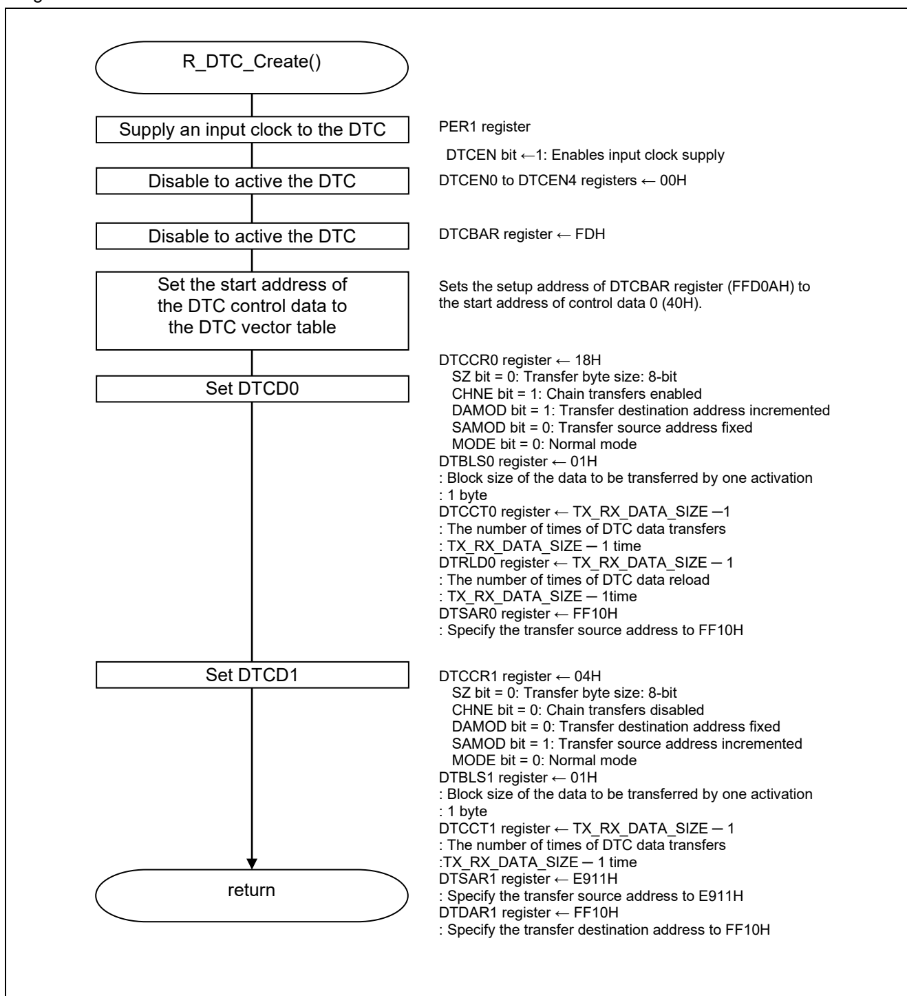
Figure 5.4 DTC Initialization
