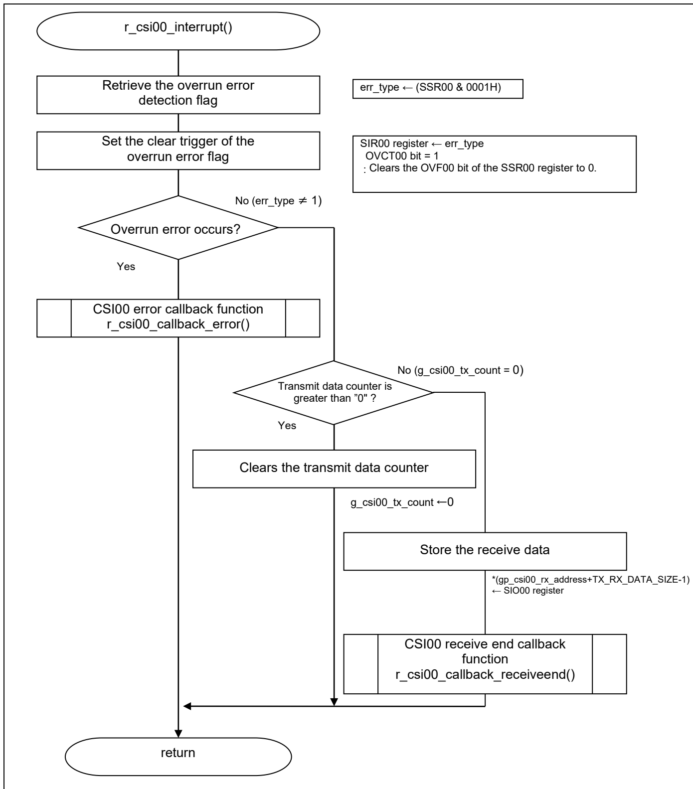
Figure 5.10 CSI00 Transfer End Interrupt
