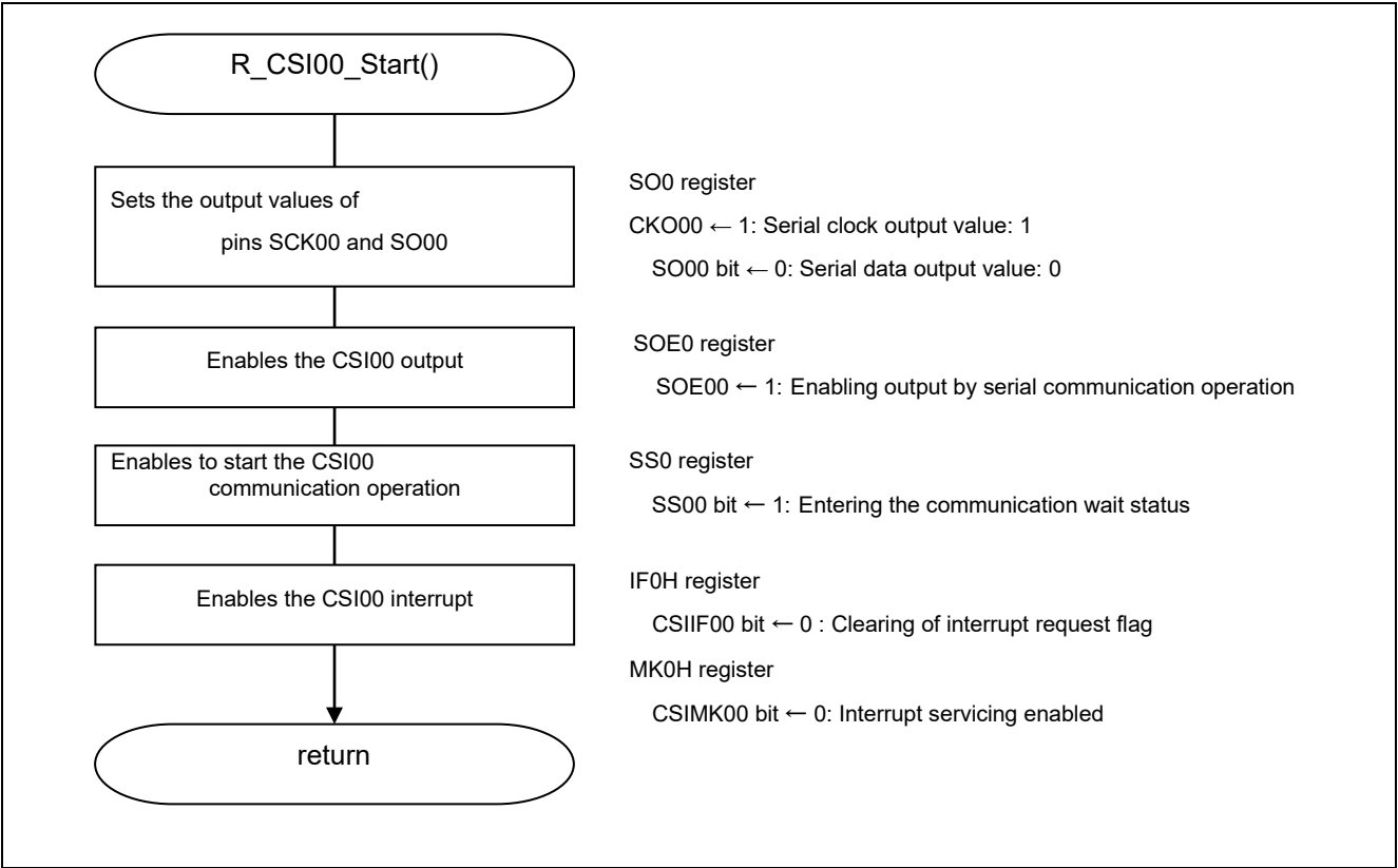
Figure 5.7 CSI00 Operation Start
