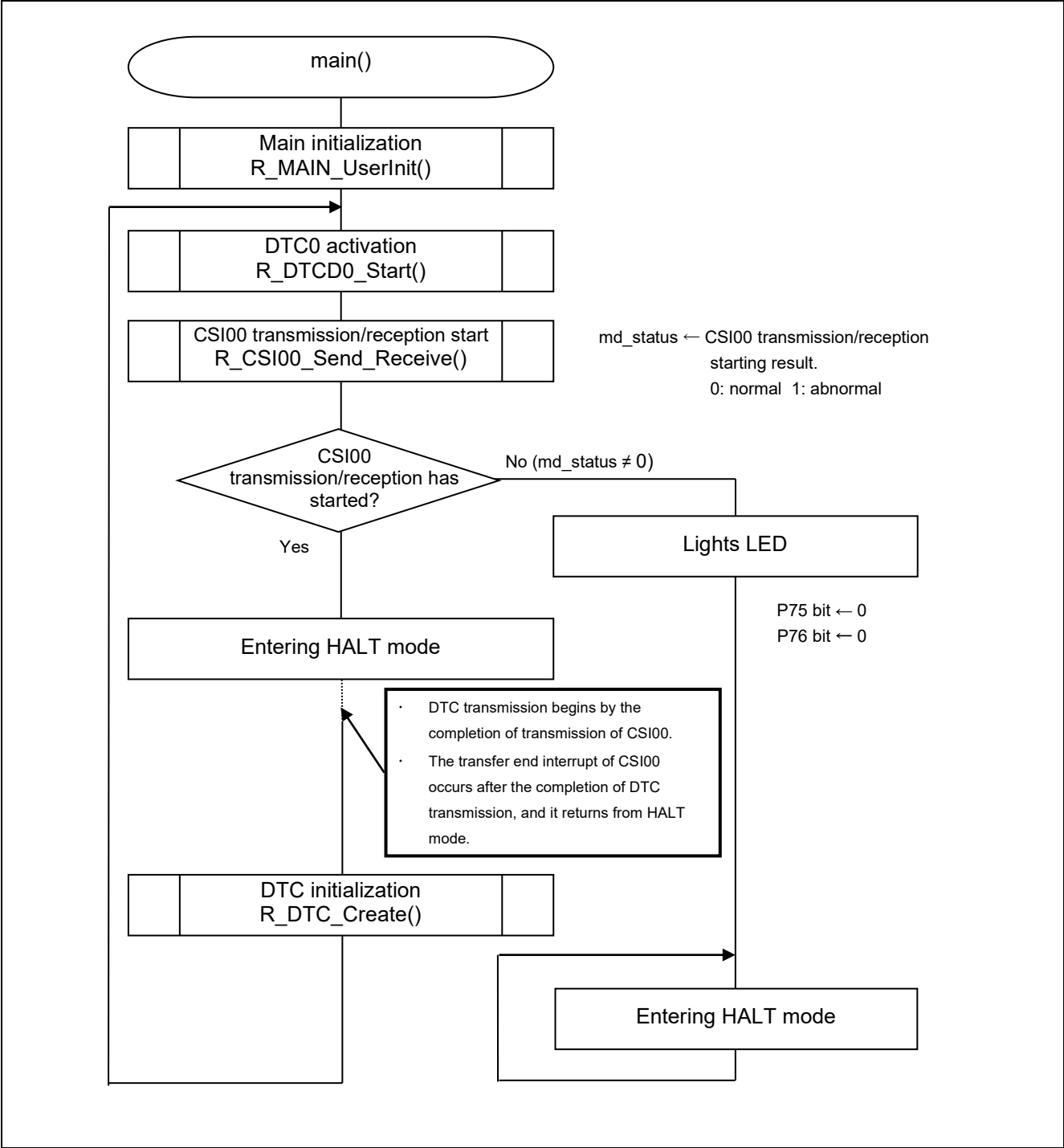
Figure 5.5 Main Processing
