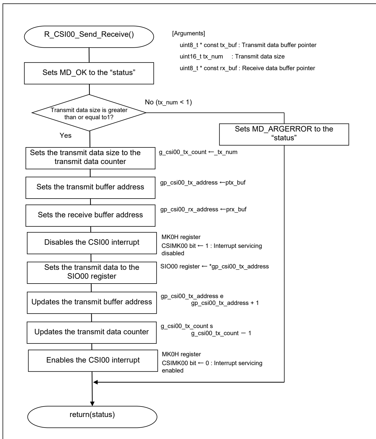
Figure 5.9 CSI00 Transmission/Reception Start
