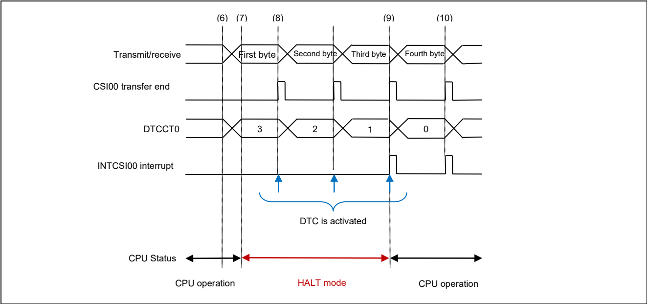
Figure 5.2 Timing of Transmission/Reception and DTC Activation
