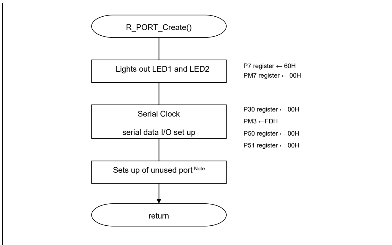
Figure 5.9 Port Initialization
