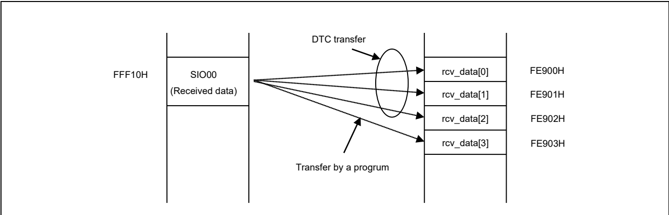
Figure 5.3 DTCD0 Operation
