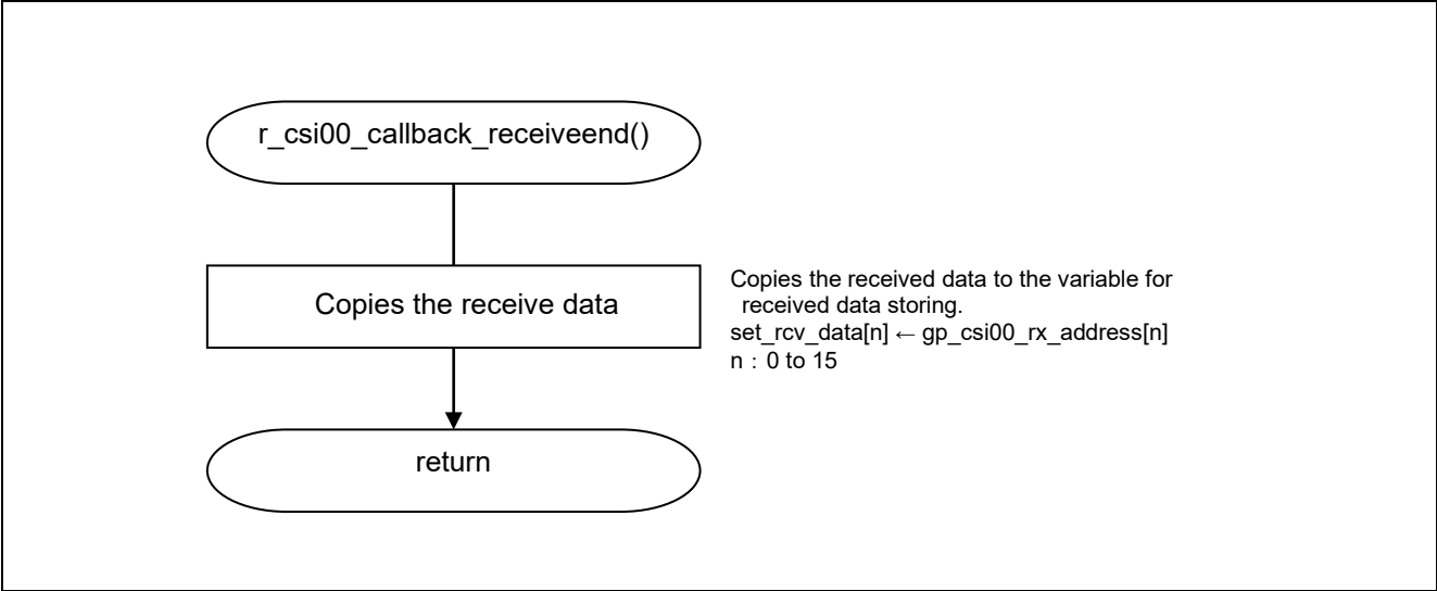
Figure 5.11 CSI00 Receive End Callback Function
