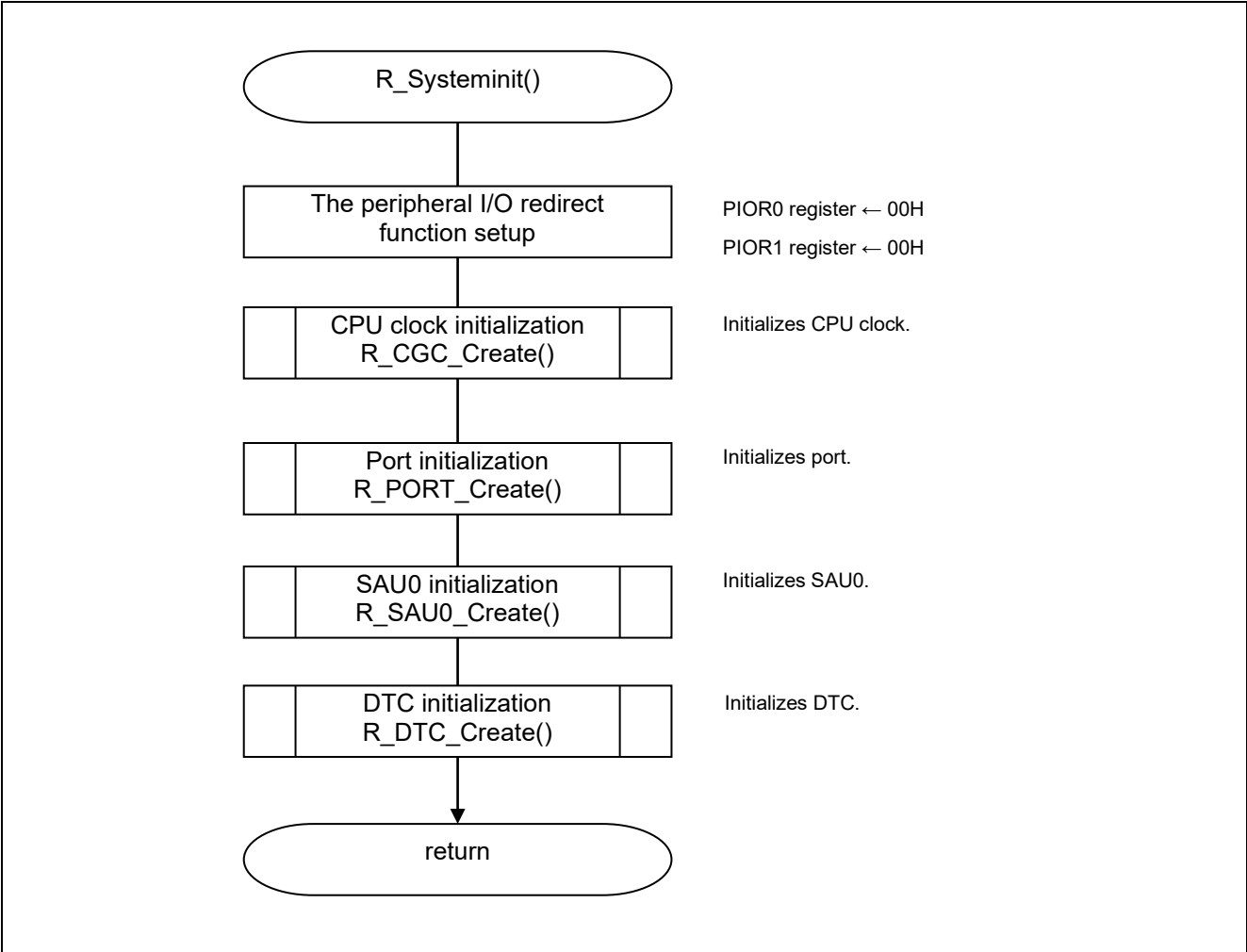
Figure 5.7 Peripheral Function Initialization
