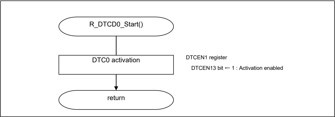
Figure 5.8 DTC0Activation
