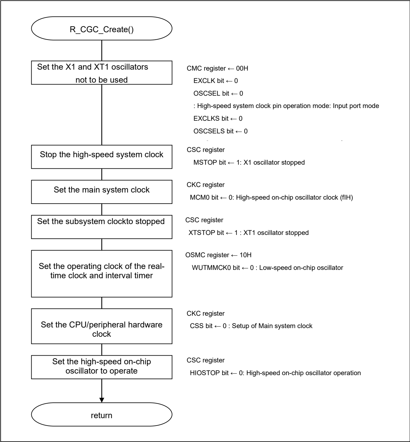
Figure 5.8 CPU Clock Initialization
