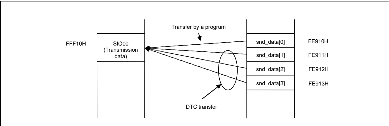
Figure 5.4 DTCD1 Operation
