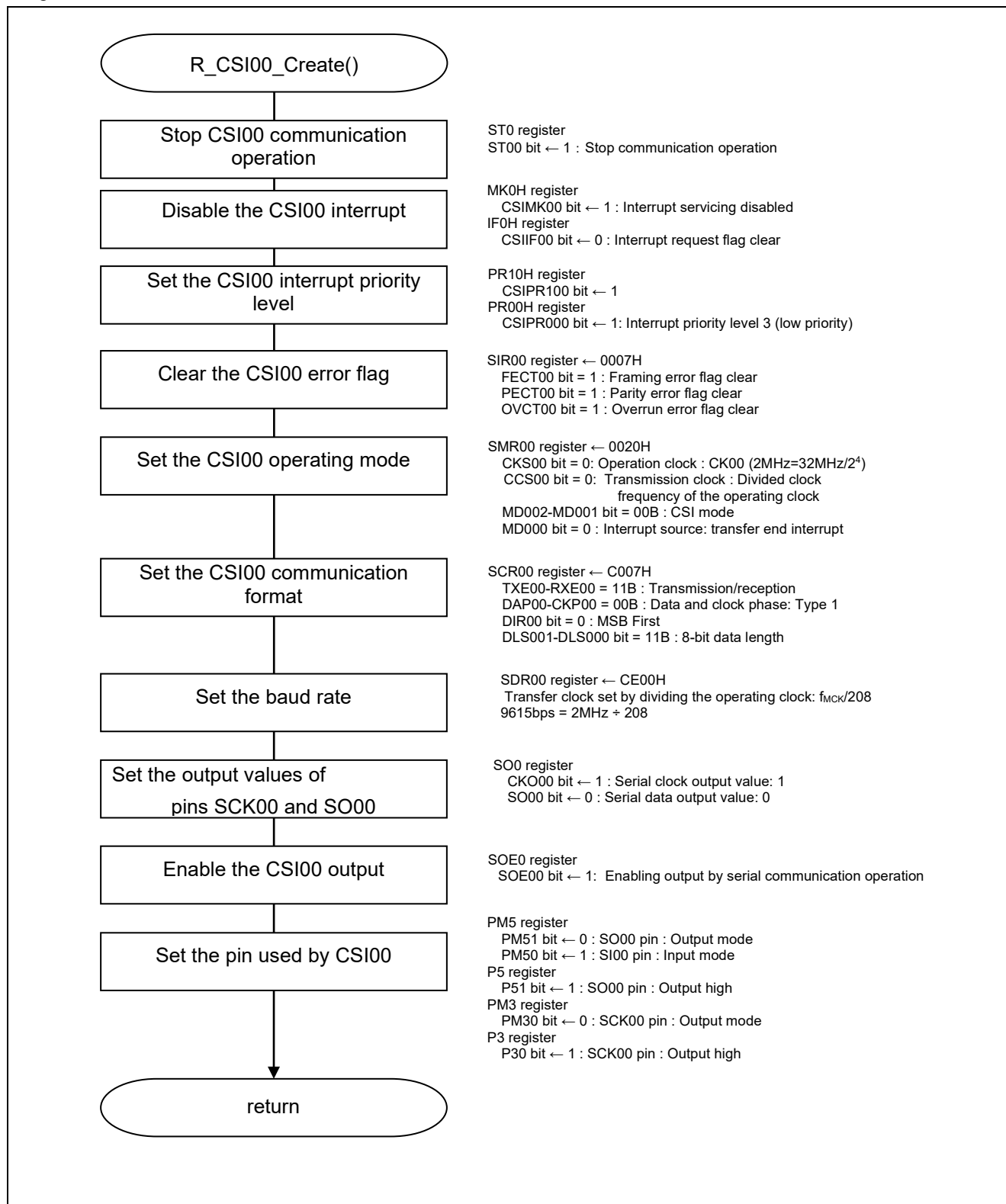
Figure 5.3 CSI00 Initialization
