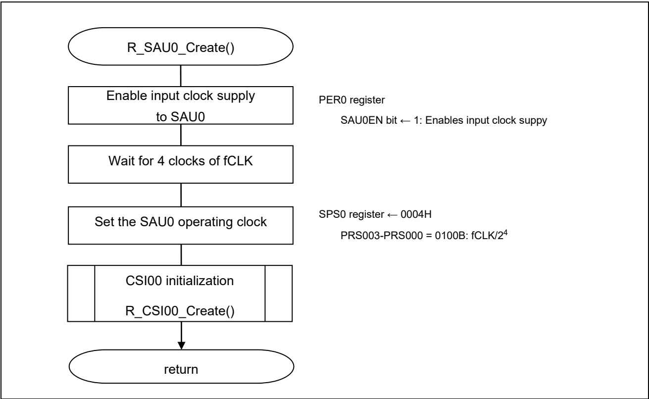
Figure 5.2 SAU0 Initialization
