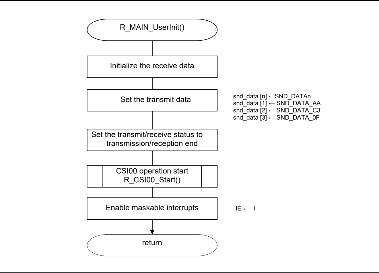
Figure 5.6 Main Initialization
