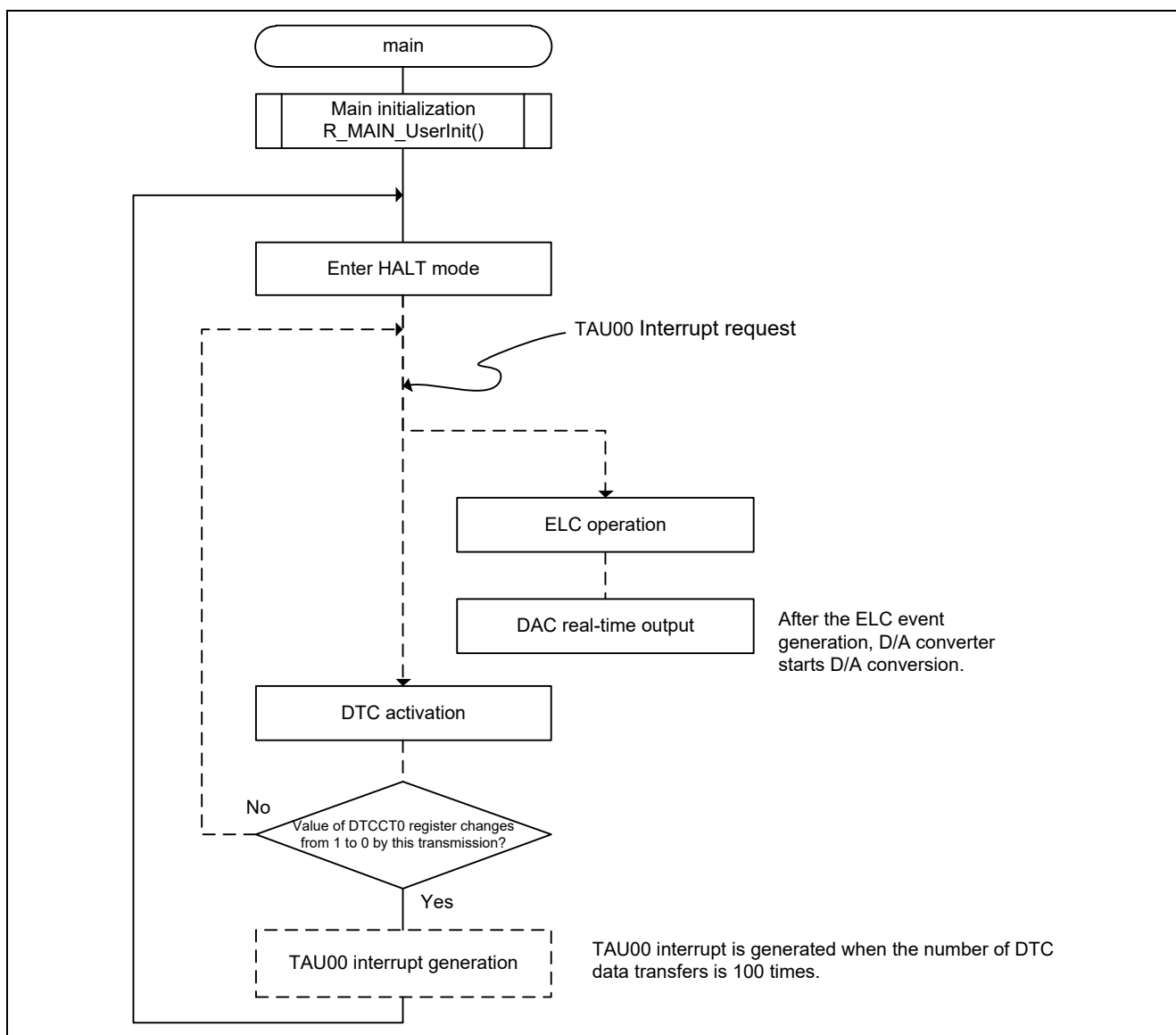
Figure 4.10 Main Processing
