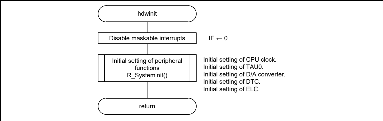
Figure 4.3 Initial Setting
