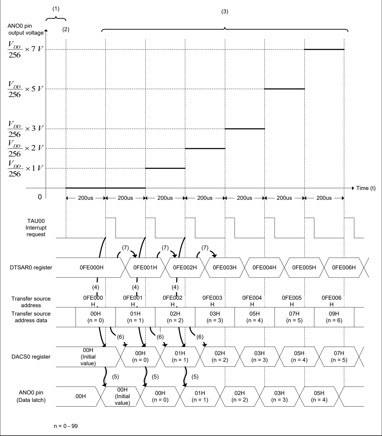
Figure 4.1 Timing Diagram
