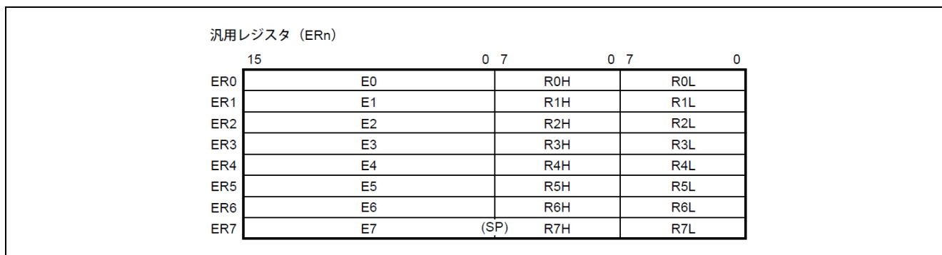
Figure 1.1 Configuration of H8/36109 general-purpose registers
