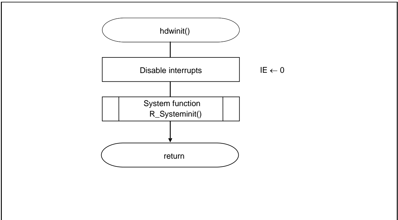
Figure 5.2 Initialization Function
