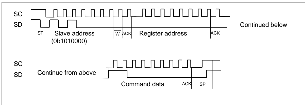
Figure 1.10 Command Setting Timing Chart
