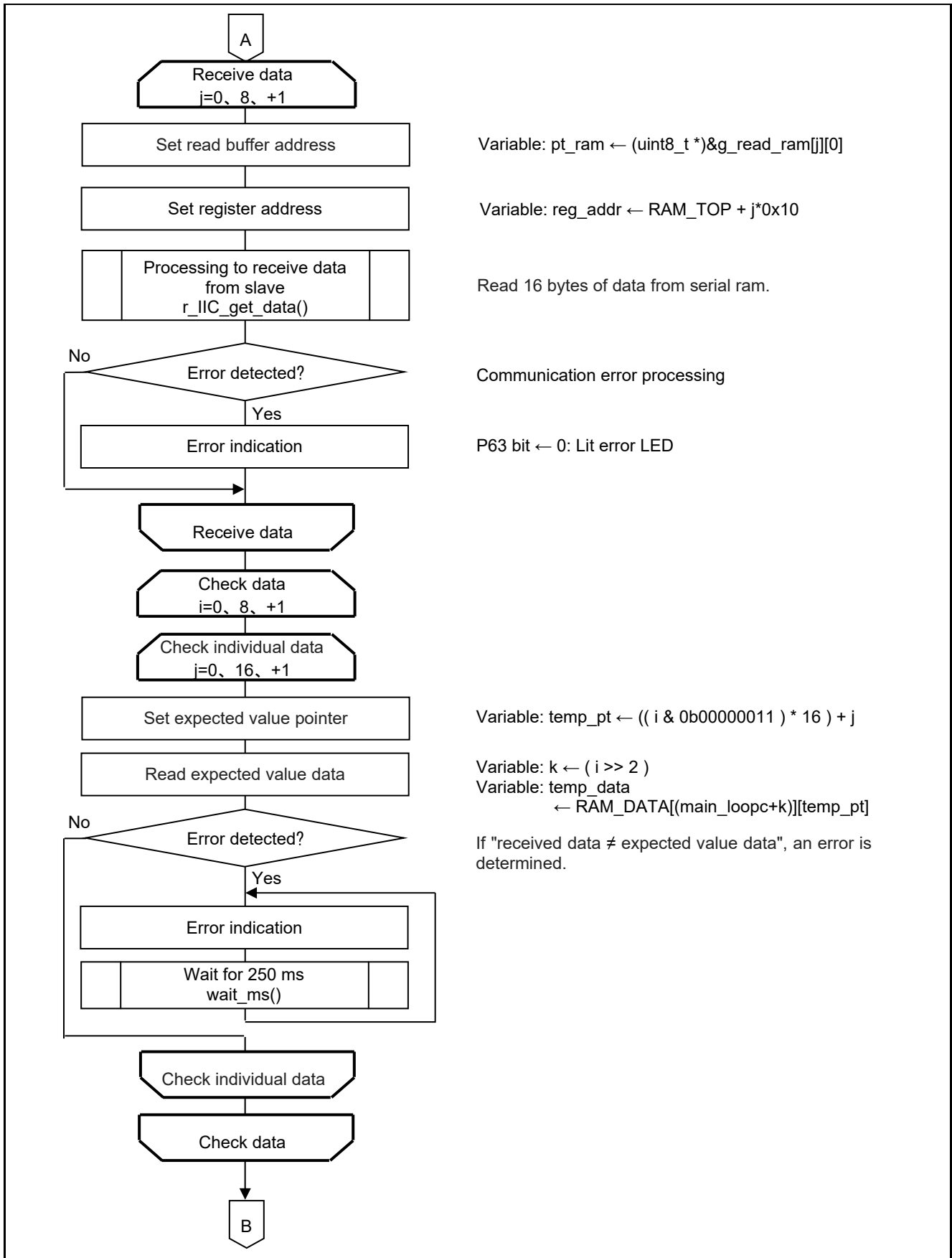
Figure 5.10 Main Processing (2/3)
