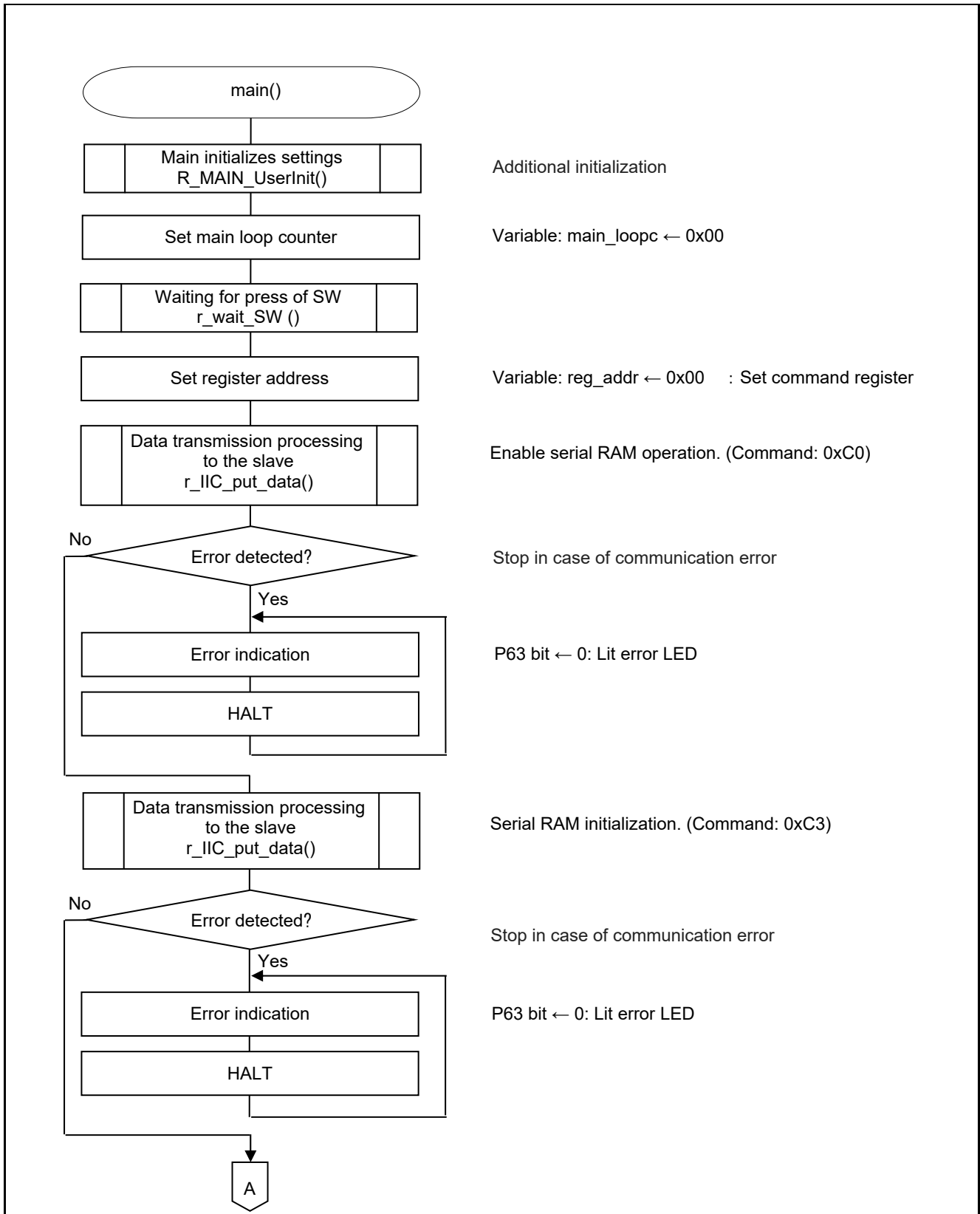
Figure 5.9 Main Processing (1/3)
