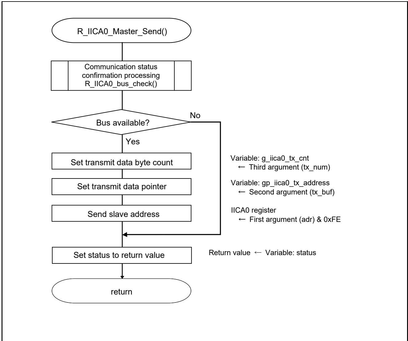
Figure 5.20 Master Transmission Start Request Processing
