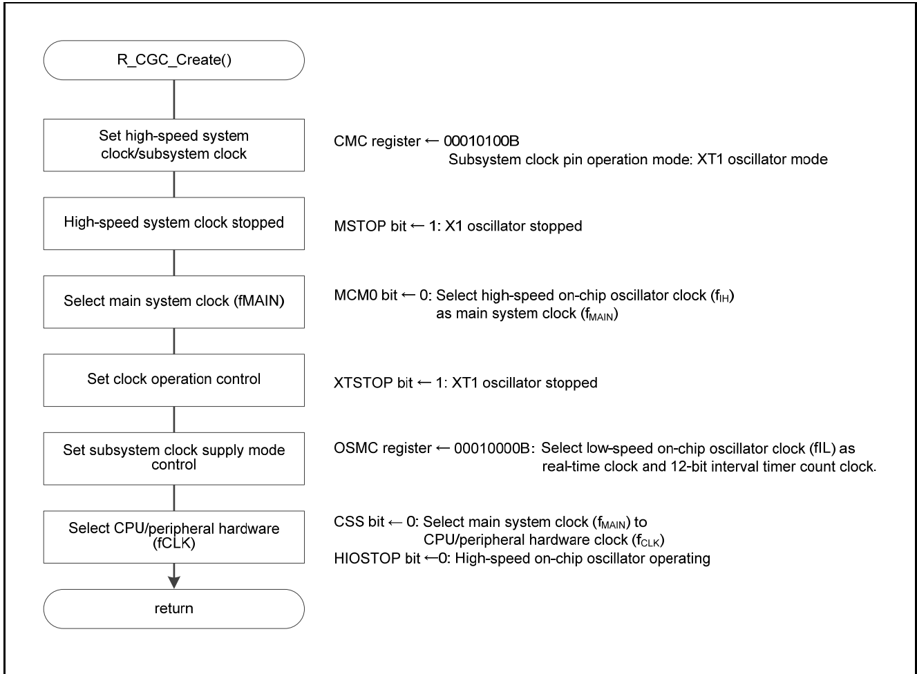
Figure 5.4 CPU Clock Setup
