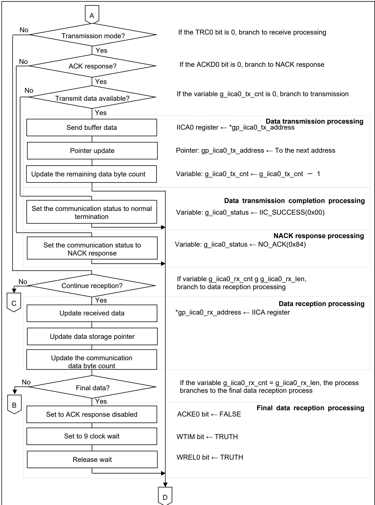
Figure 5.27 IICA0 Interrupt Processing (2/3)
