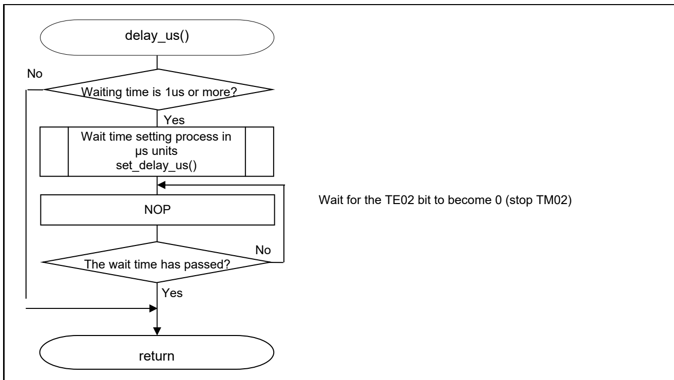
Figure 5.29 Time Wait Processing In \mu s units
