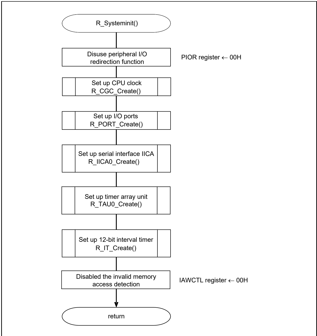
Figure 5.3 System Function
