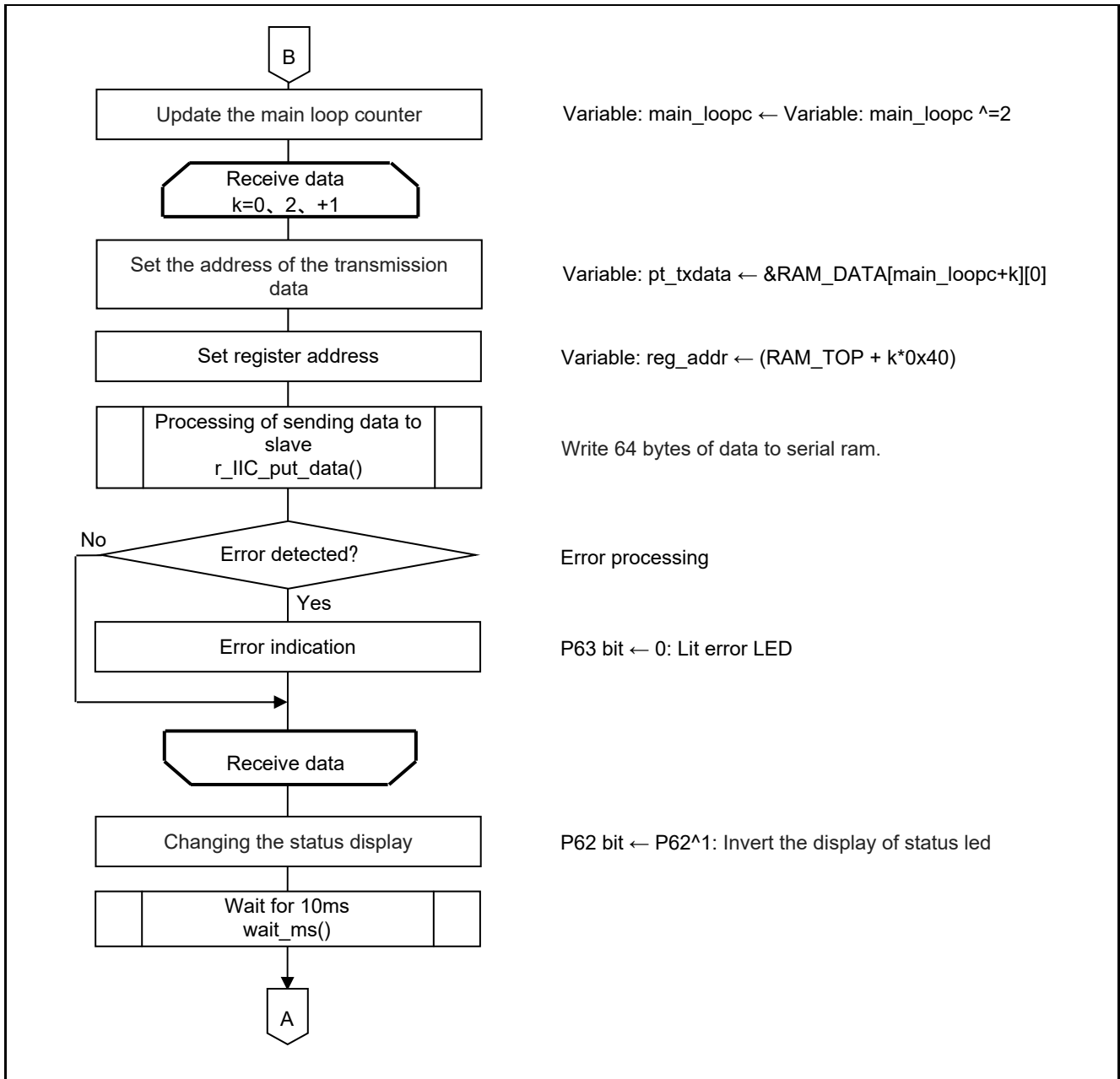
Figure 5.11 Main Processing (3/3)
