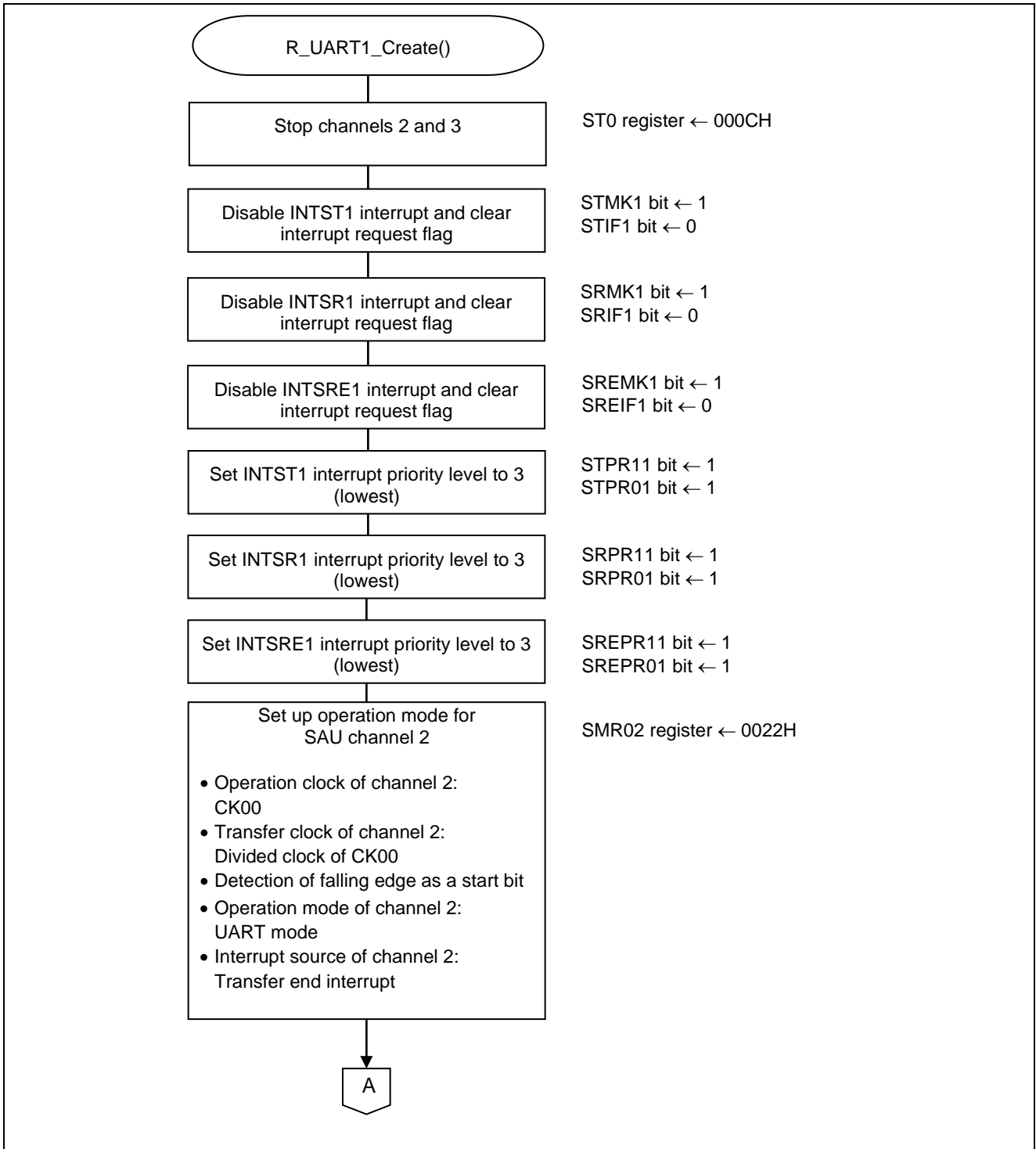
Figure 5.7 UART1 Setup (1/3)
