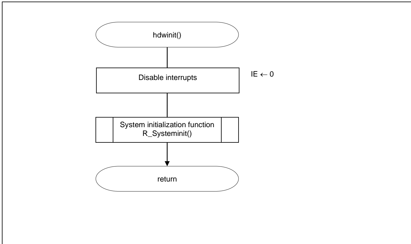
Figure 5.2 Initialization Function
