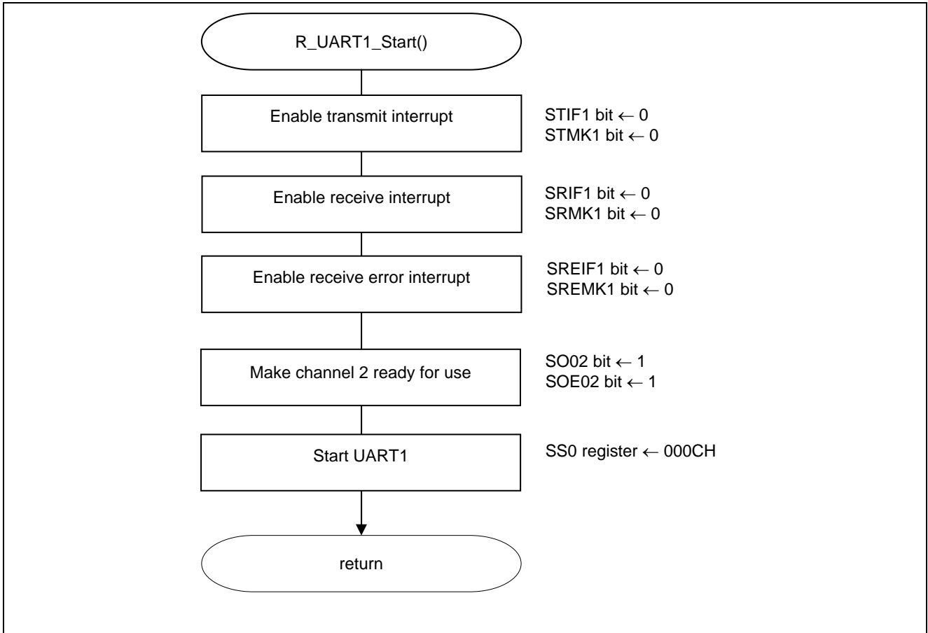
Figure 5.12 Starting the UART1
