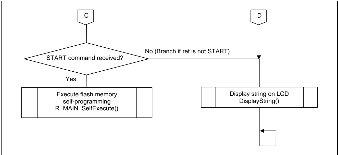
Figure 5.11 Main Processing (2/2)
