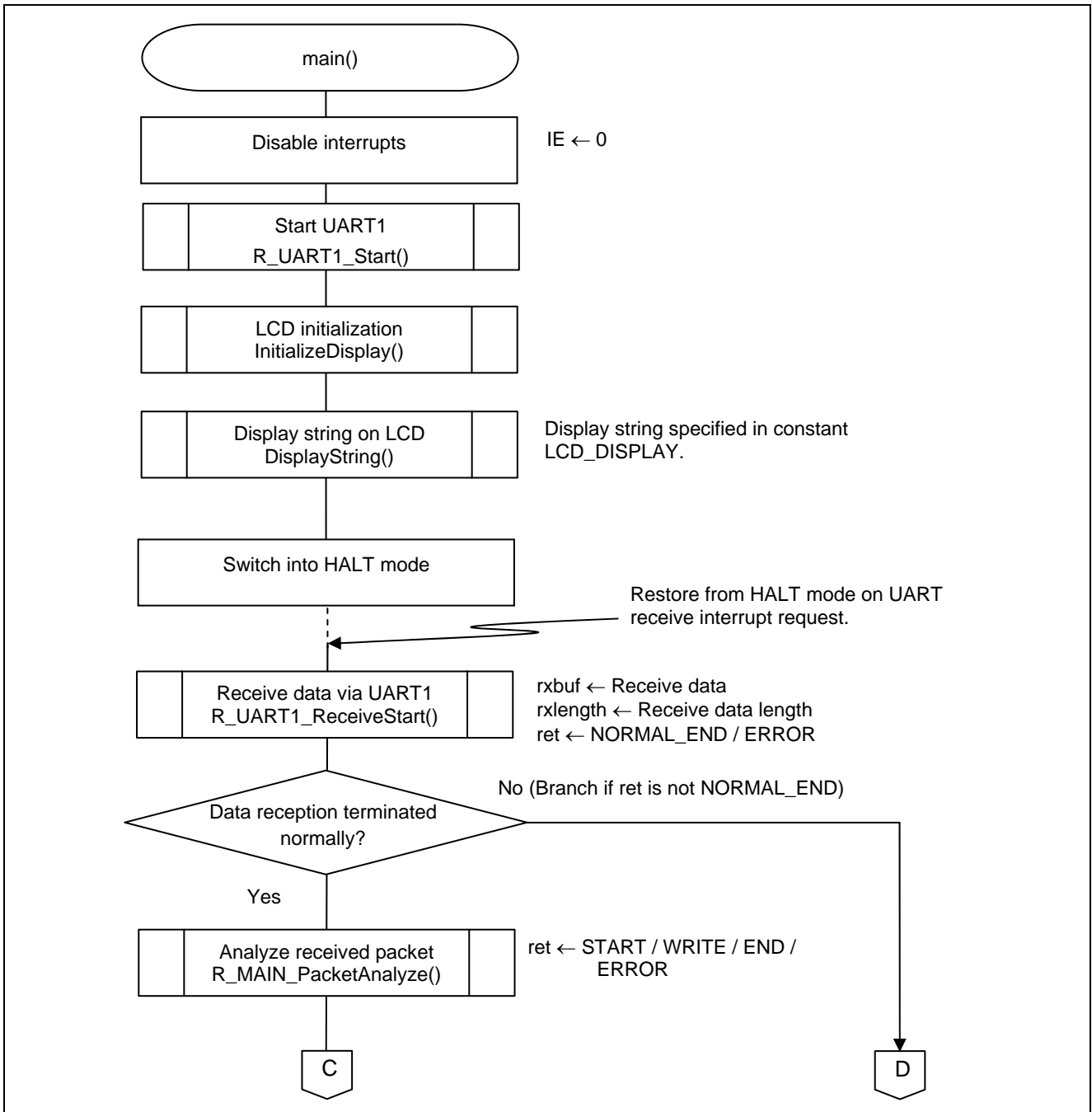
Figure 5.10 Main Processing (1/2)
