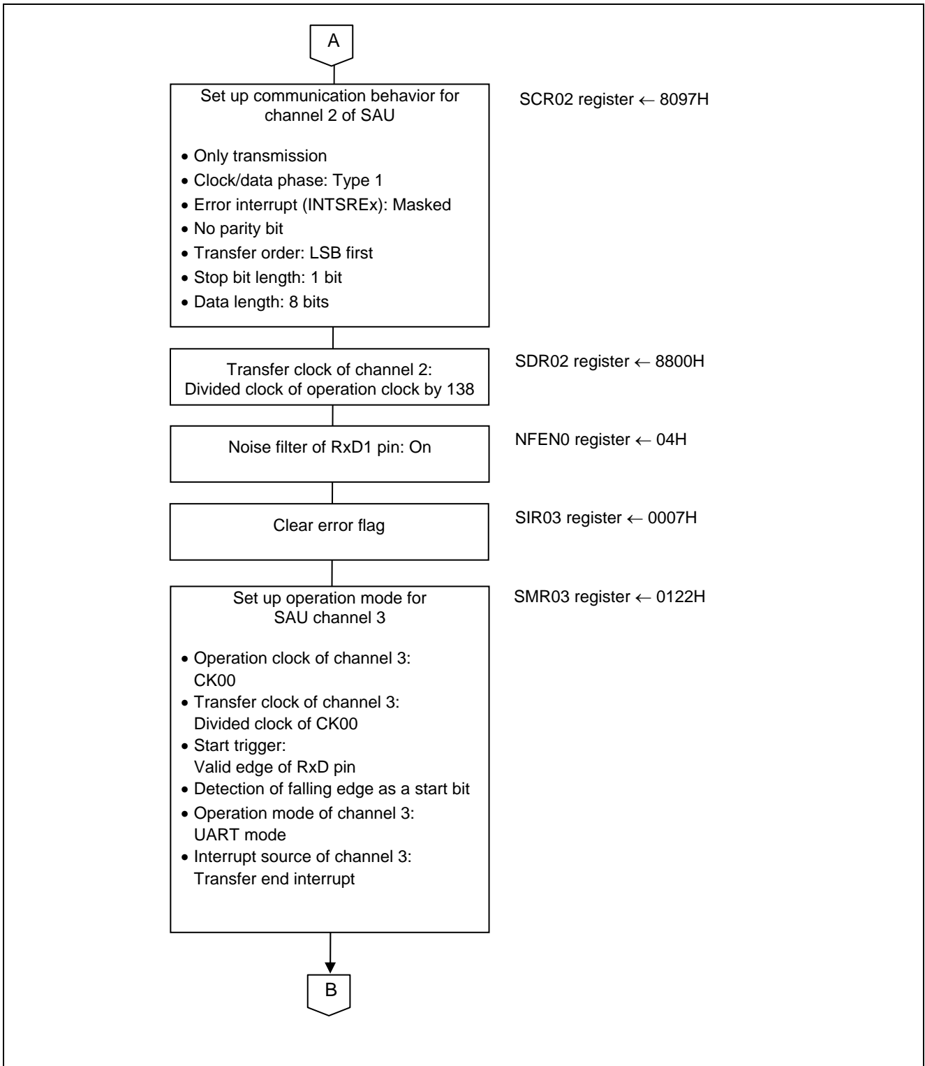
Figure 5.8 UART1 Setup (2/3)
