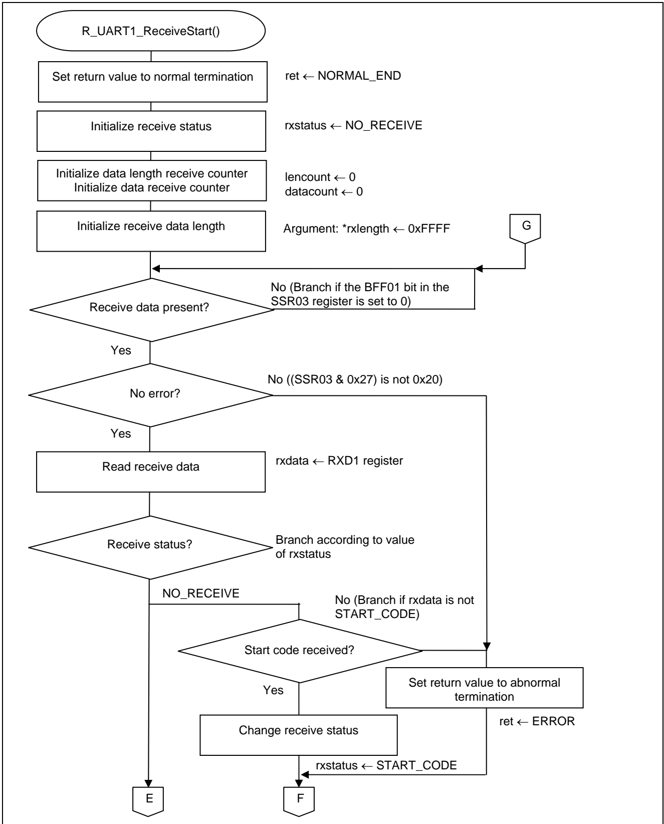
Figure 5.13 Data Reception via UART1 (1/2)
