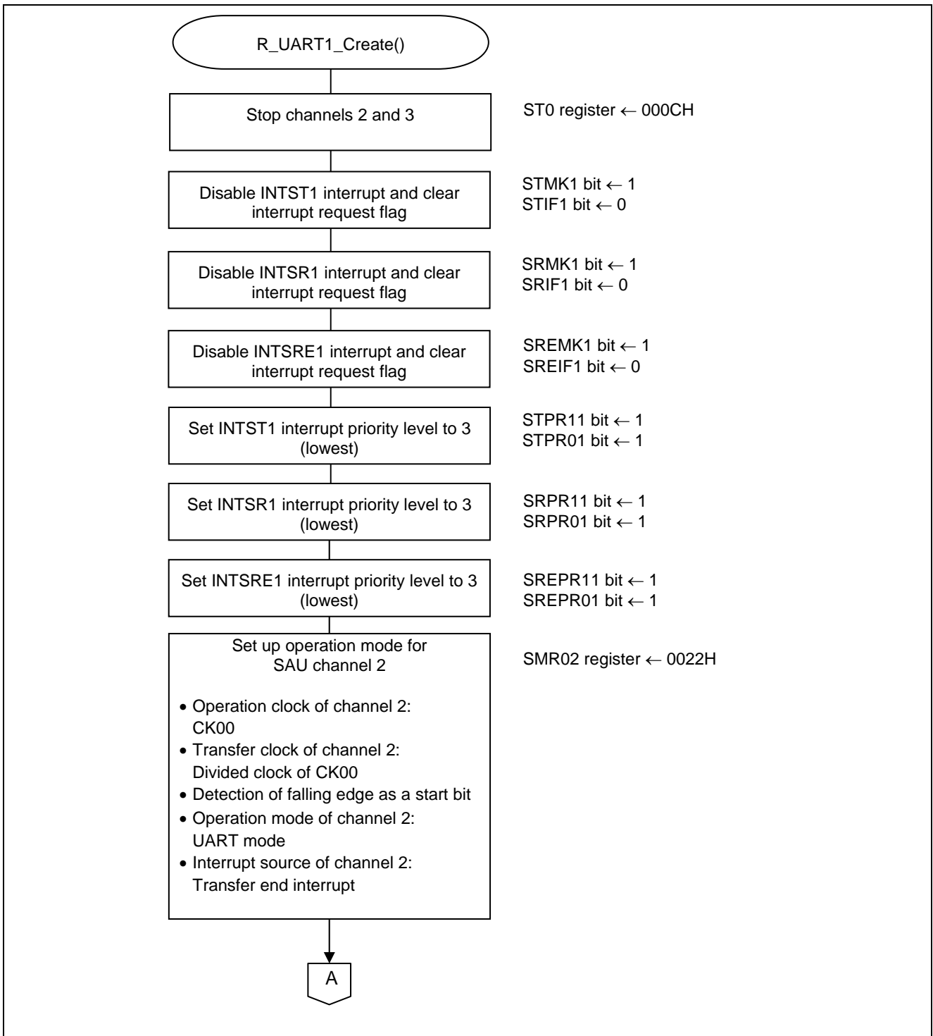
Figure 5.7 UART1 Setup (1/3)
