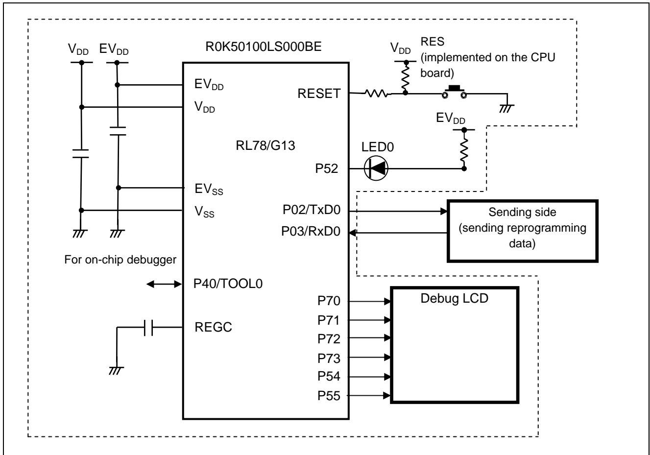
Figure 4.1 Hardware Configuration
