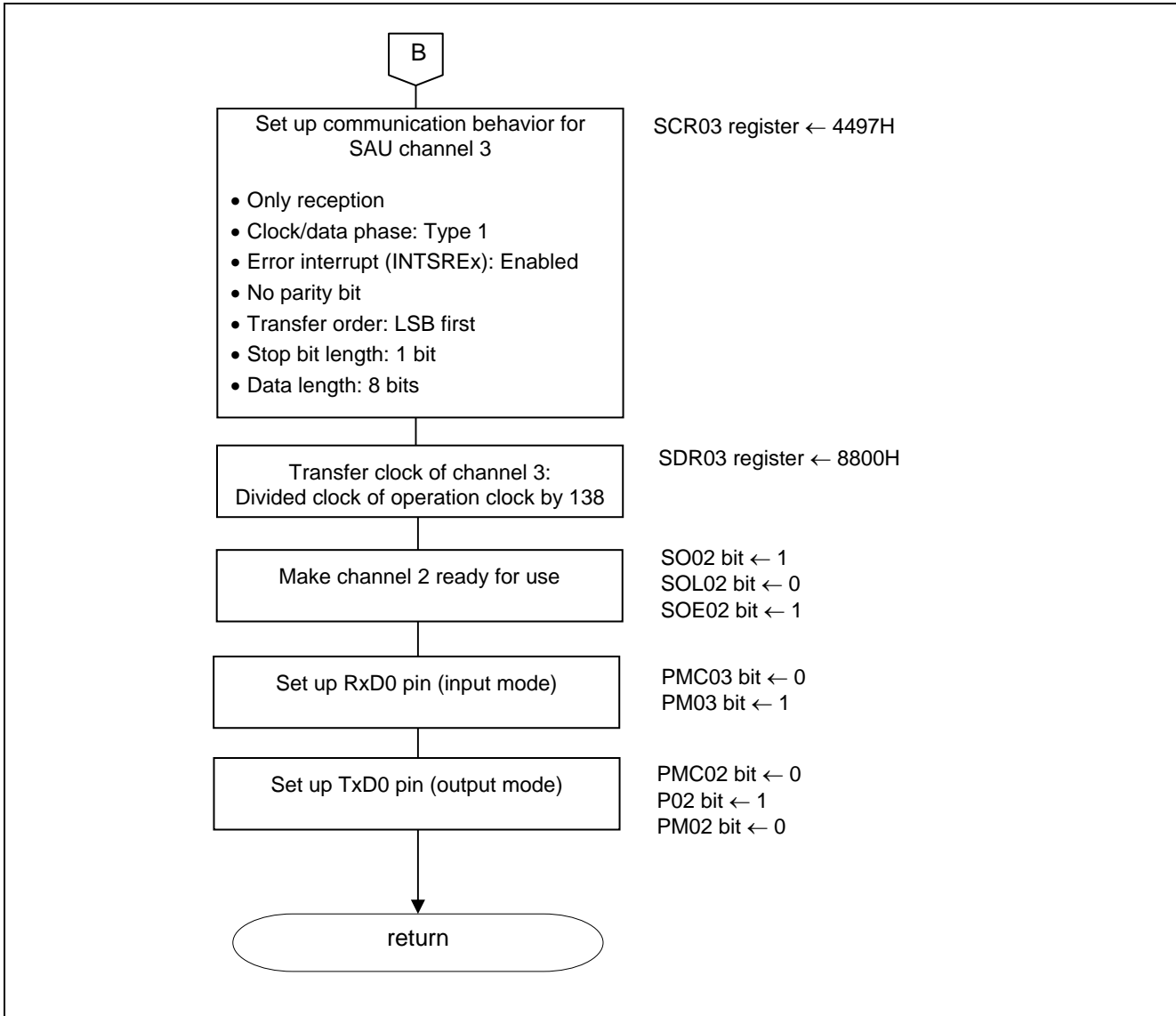
Figure 5.9 UART1 Setup (3/3)
