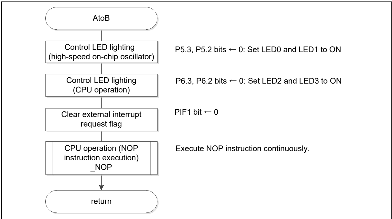
Figure 5.9 Status Transition AtoB
