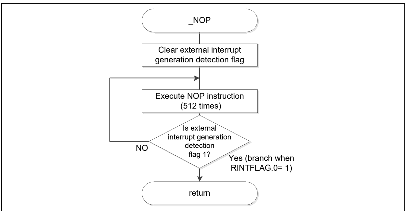
Figure 5.10 CPU Operation (NOP instruction execution)
