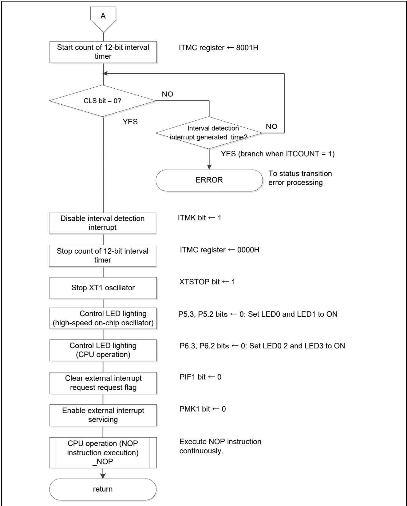
Figure 5.17 Status Transition DtoB (2/2)
