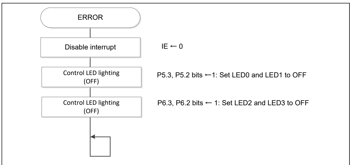
Figure 5.13 Error Processing of Status Transition
