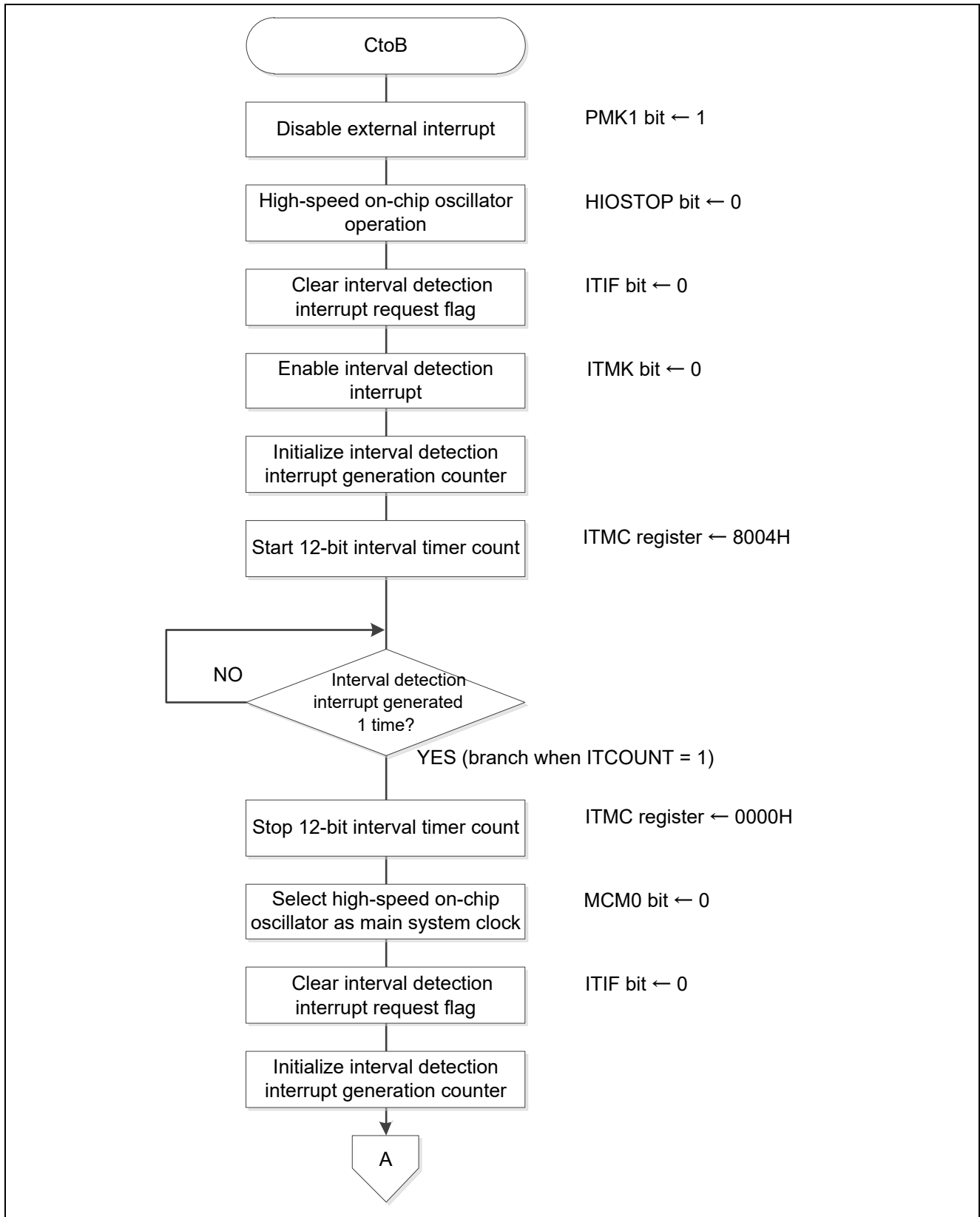
Figure 5.28 Status Transition CtoB (1/2)
