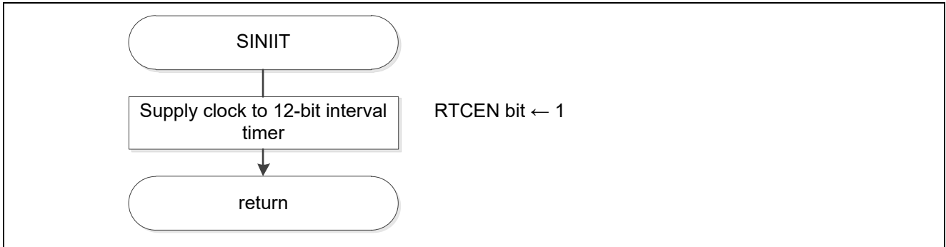
Figure 5.6 12-bit Interval Timer Setting
