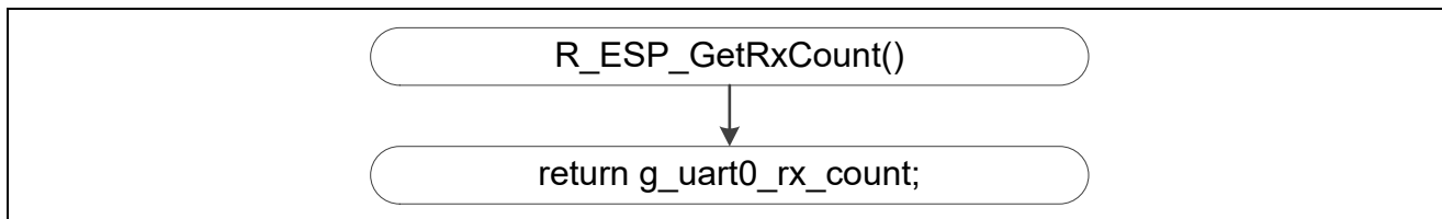
Figure 4.20 Getting the Length of Data Received through UART
