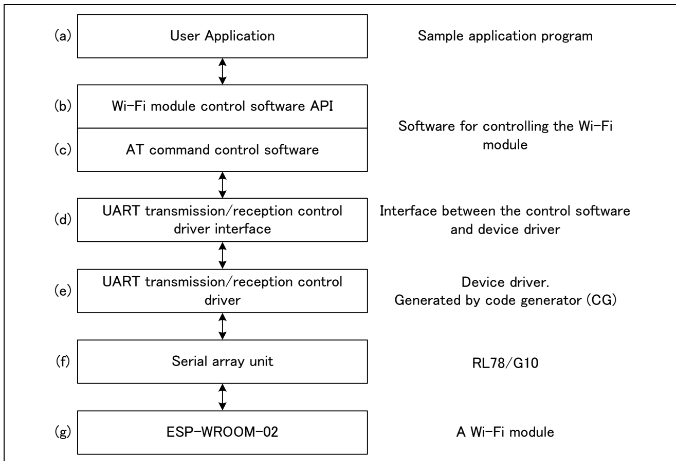
Figure 4.1 Example of Software Configuration
