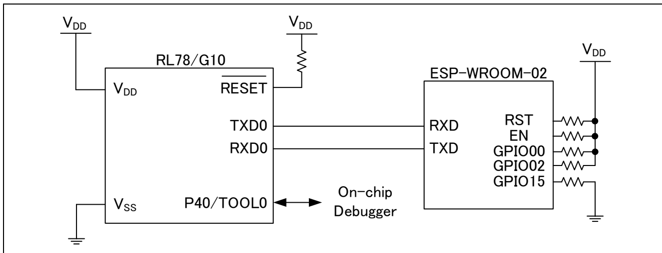
Figure 3.1 Hardware Configuration
