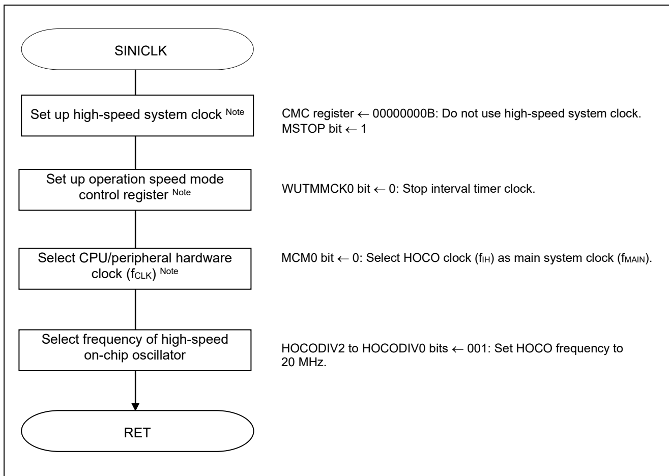
Figure 5.4 Clock Generation Circuit Setup
