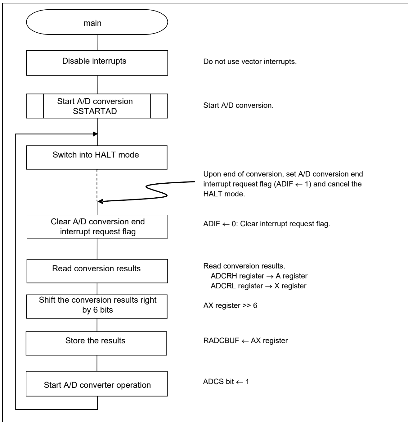
Figure 5.6 Main Processing
