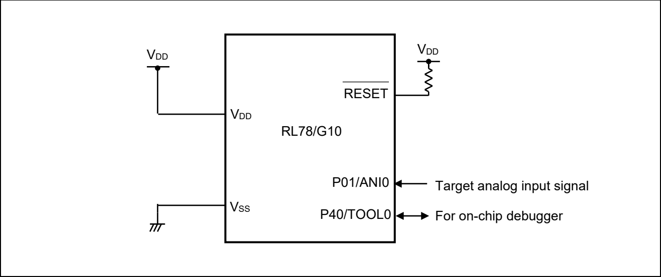
Figure 4.1 Hardware Configuration
