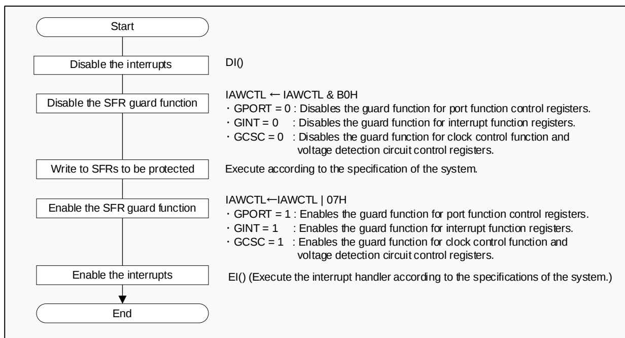
Figure 8-1 Example of Using SFR Guard Function
