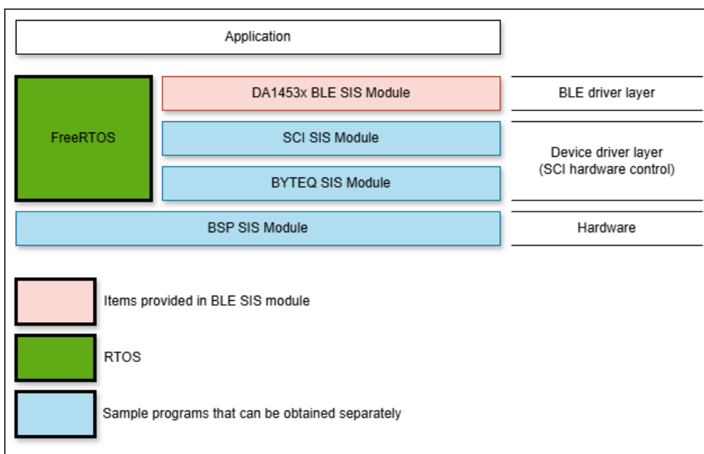
Figure 1.2 Software Configuration Diagram
