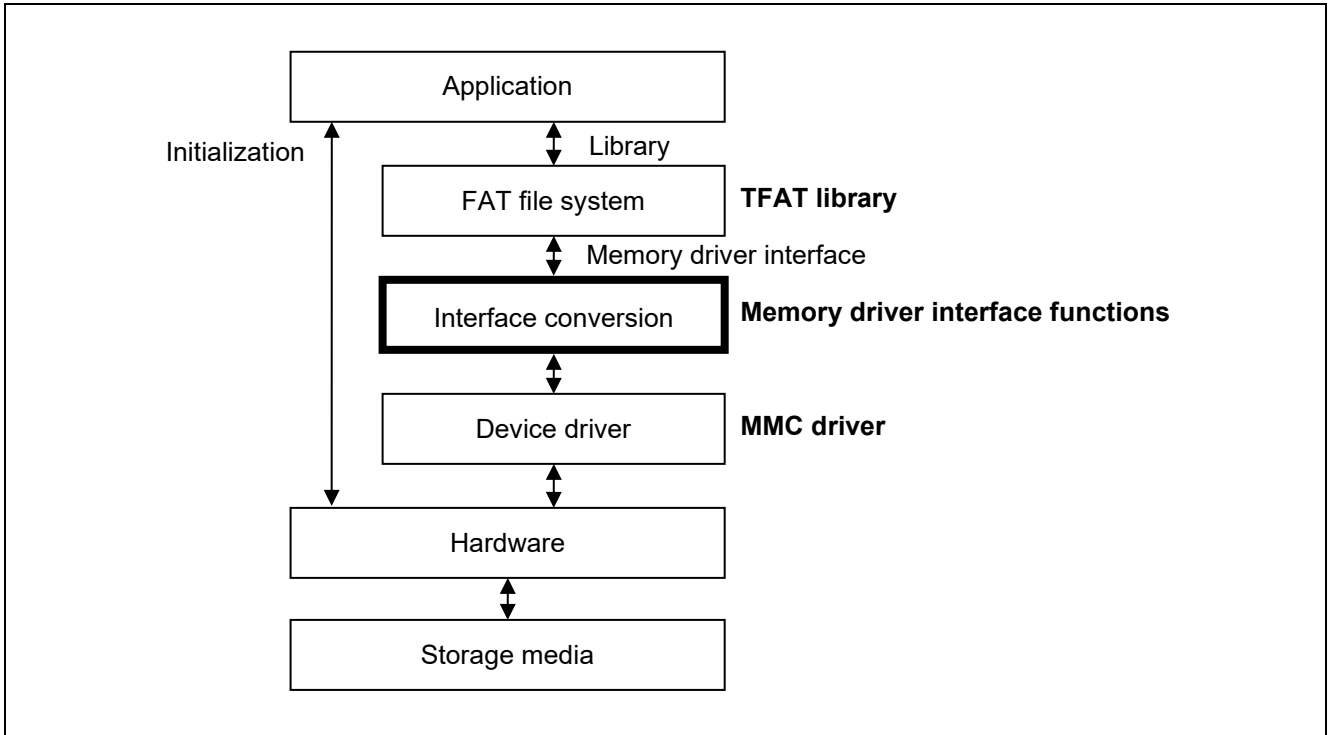
Figure 4.1 Configuration of TFAT Library and MMC Driver
